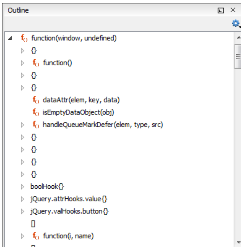
Figure 127. JavaScript Outline View
