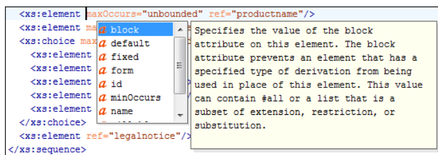
Figure 182: Content Completion Assistant
