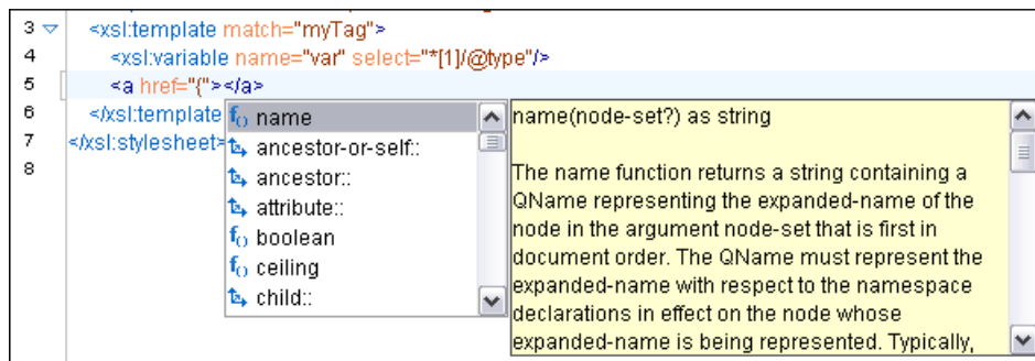
Figure 237: Content Completion in Attribute Value Templates
