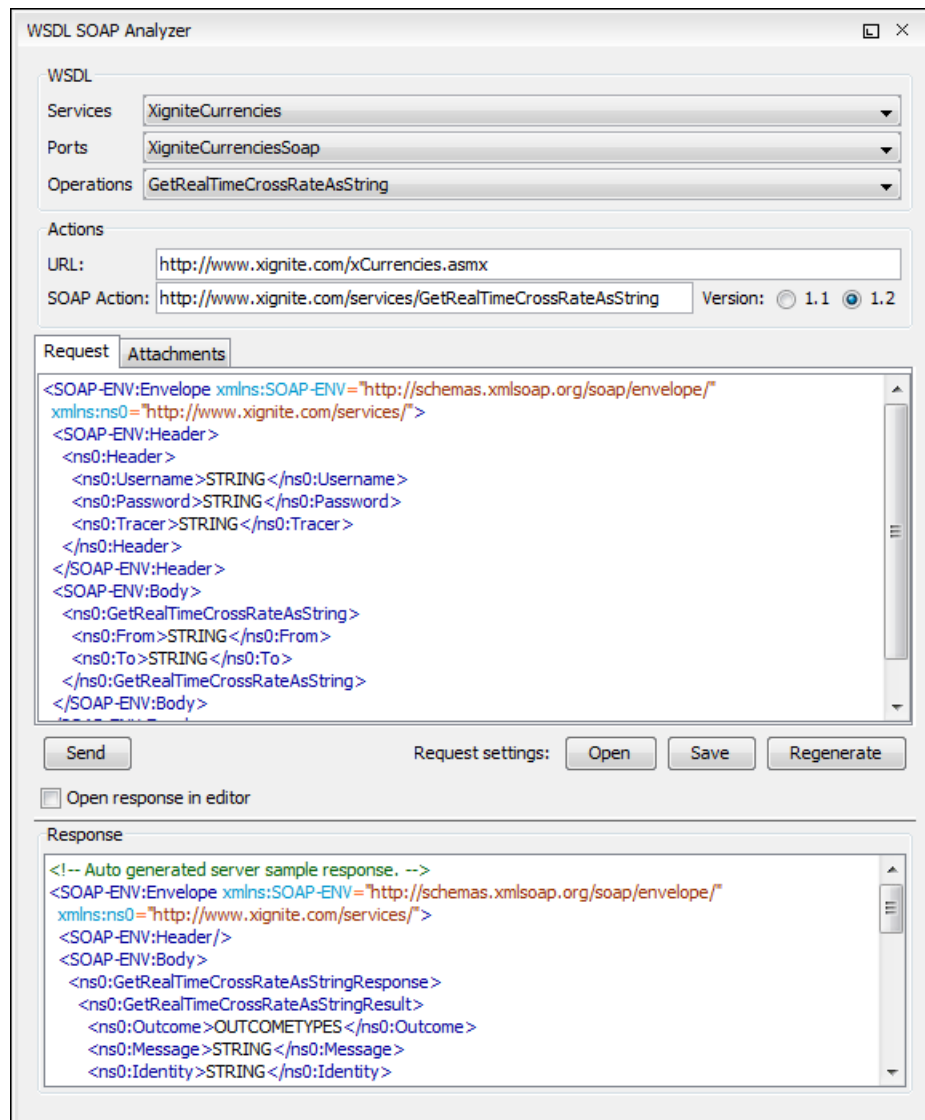
Figure 360: WSDL SOAP Analyzer Dialog Box
