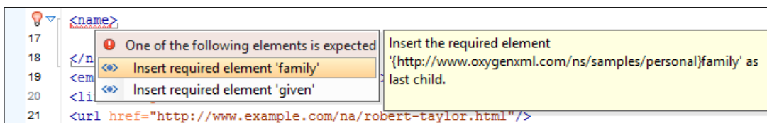
Figure 207: Quick Fix Menu Invoked by Clicking on the 💡 Icon
