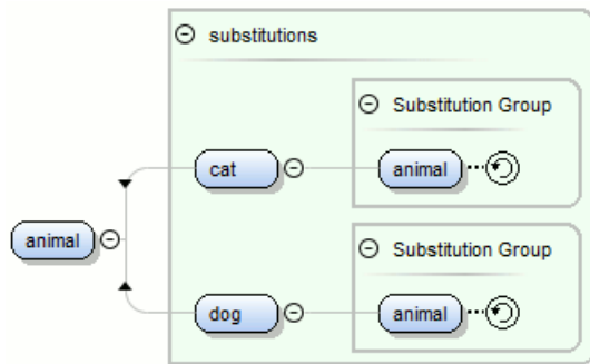
Figure 113: Substitutions Construct
