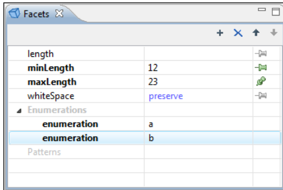
Figure 263: Facets View
