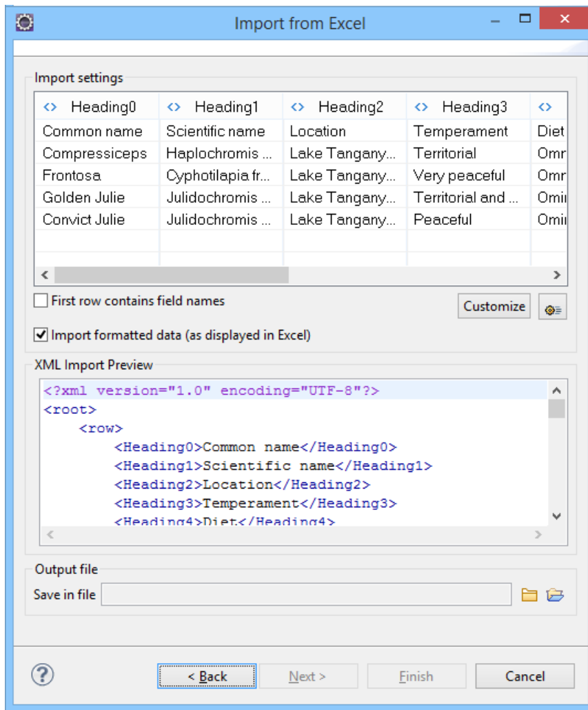
Figure 424: Import Wizard
