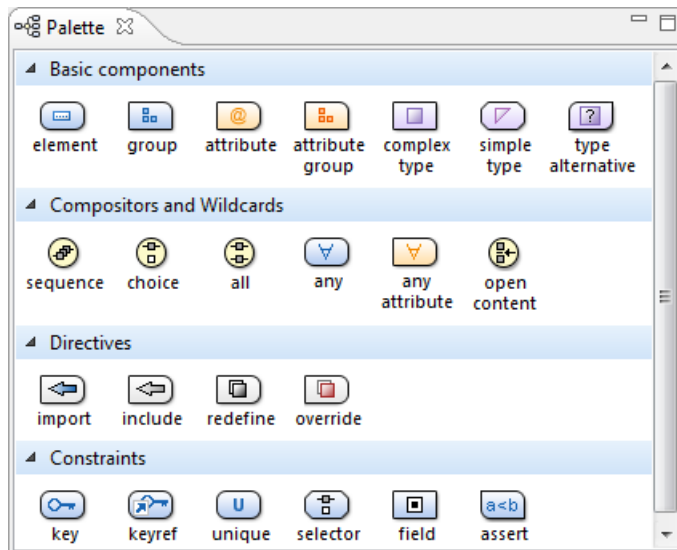
Figure 262: Palette View
