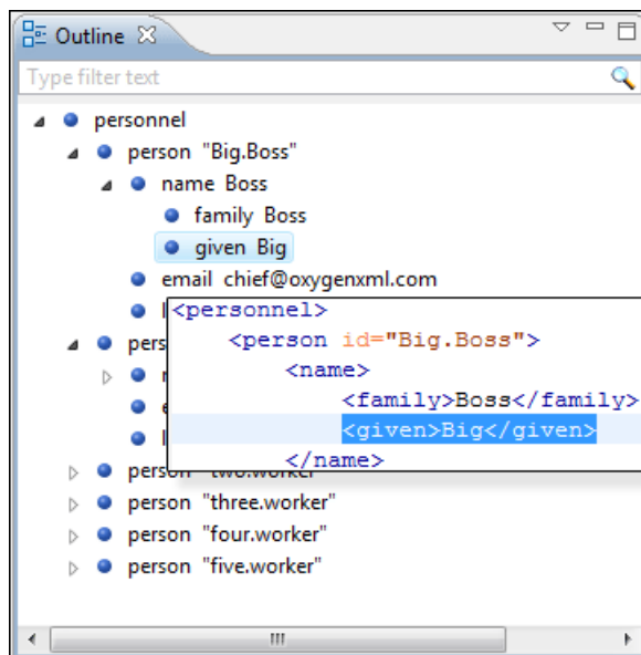
Figure 144: Outline View in Text Mode
