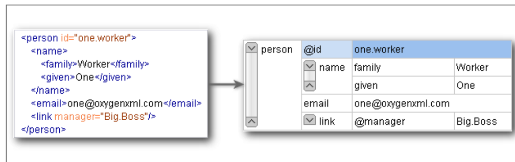
Figure 64: Pasting XML Data into Grid
