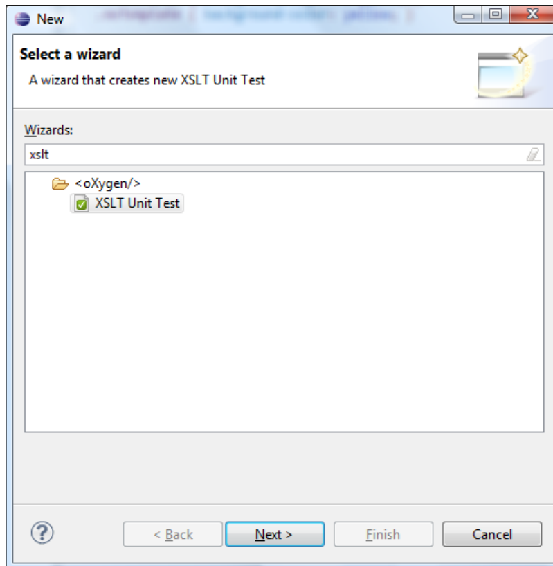
Figure 207: New XSLT Unit Test Wizard
