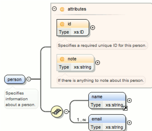
Figure 76: Extracting a Global Attribute
