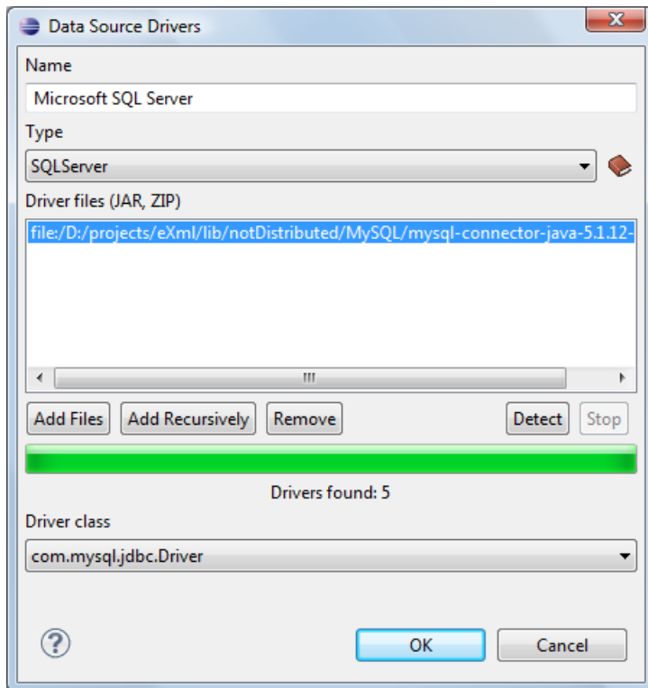
Figure 399: Data Source Drivers Configuration Dialog Box
