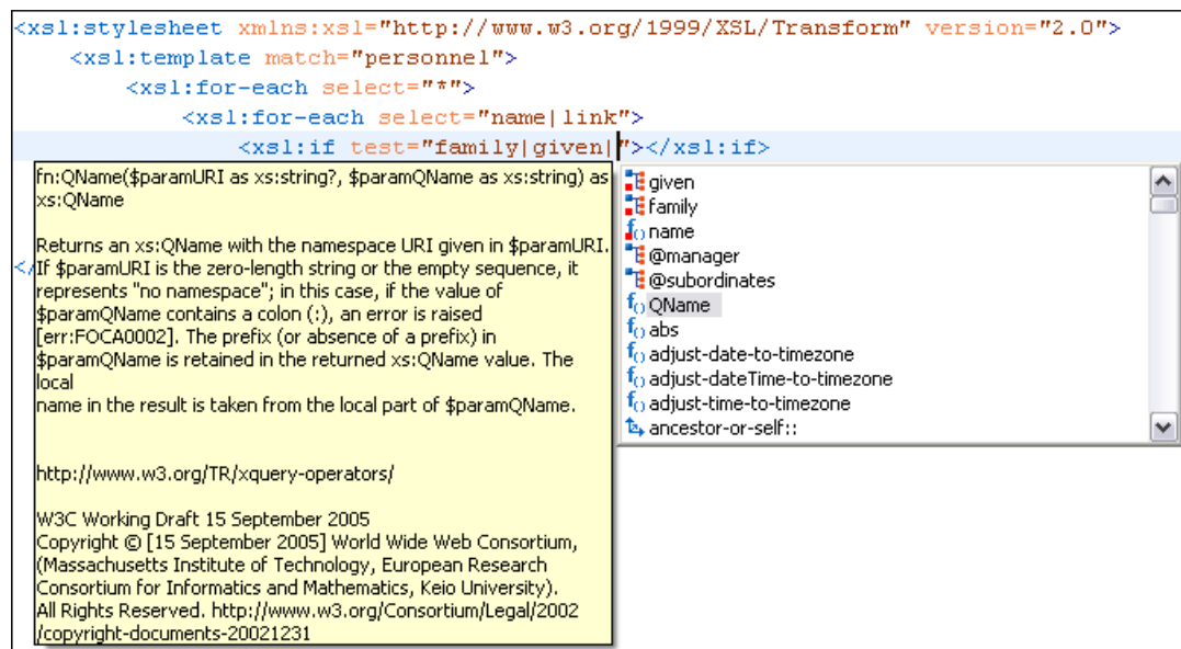
Figure 188: Content Completion in the test Attribute
