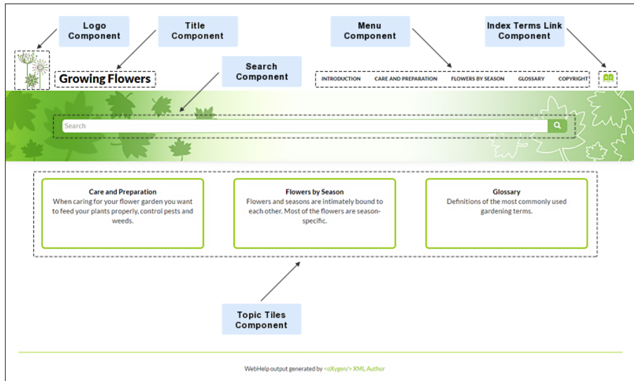
Figure 375: Examples of Main Page Components for a Tiles Style of Layout
