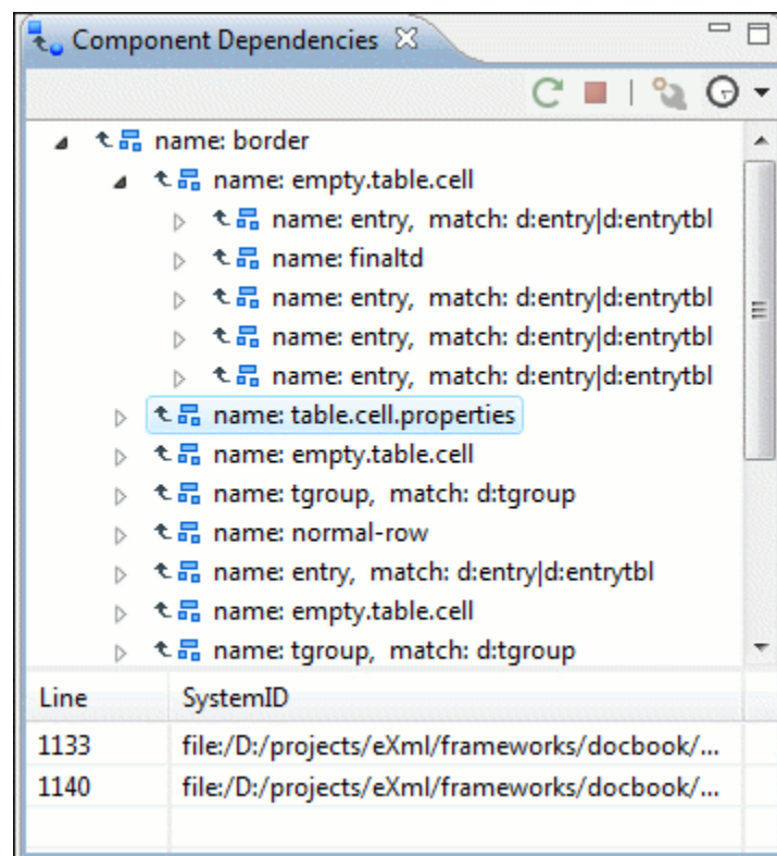
Figure 203: Component Dependencies View - Hierarchy for table.xsl
