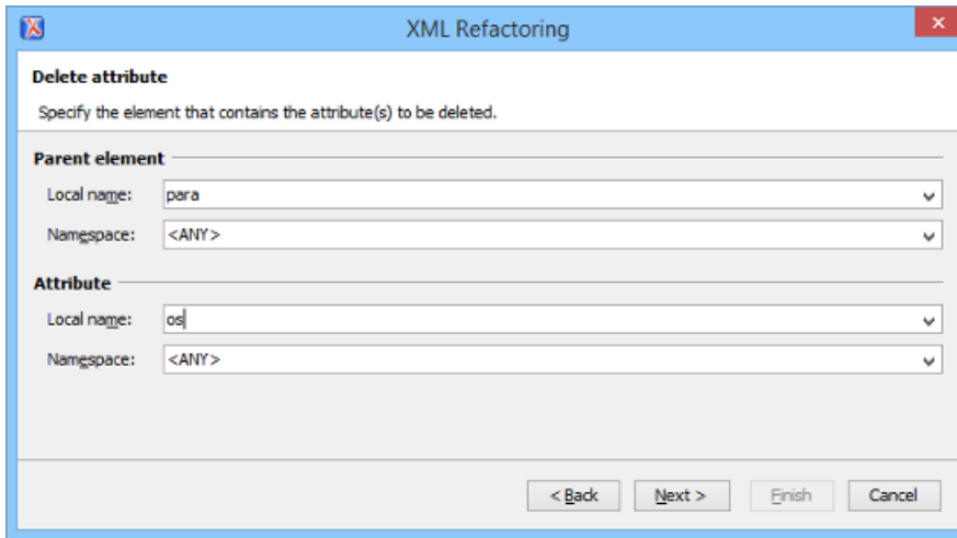
Figure 445: XML Refactoring 2nd Wizard Page (Delete Attribute Operation)
