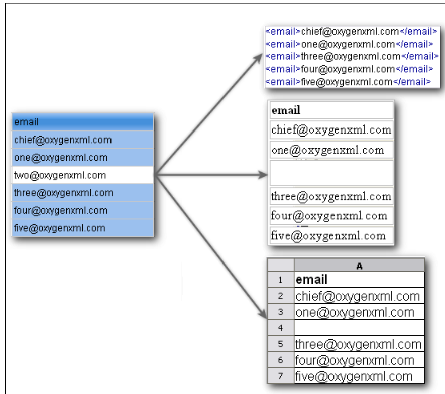
Figure 63: Copying from Grid to Other Editors
