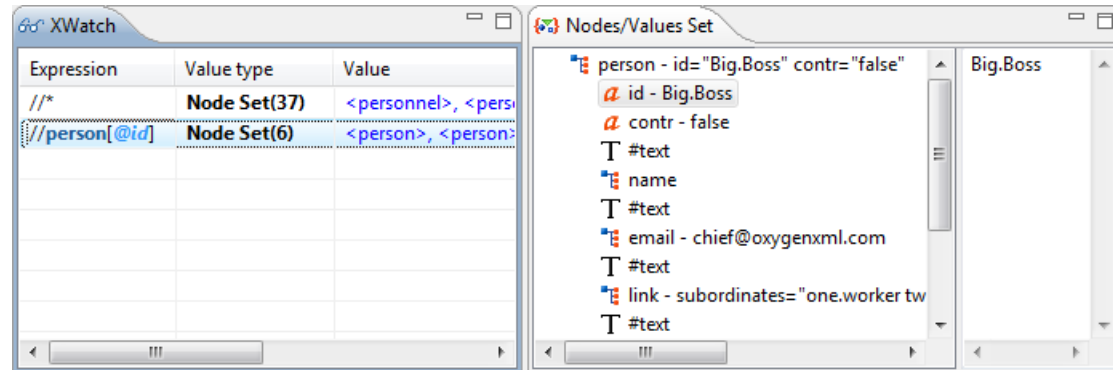
Figure 431: XPath Watch View
