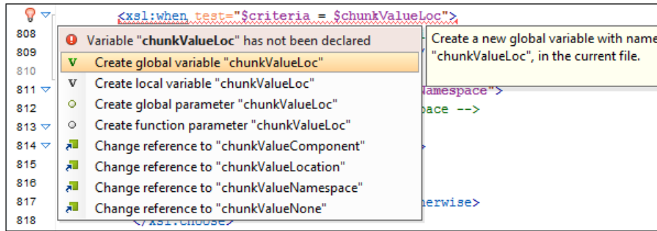
Figure 183: Example of an Undeclared XSLT Variables/Parameters Quick Fix
