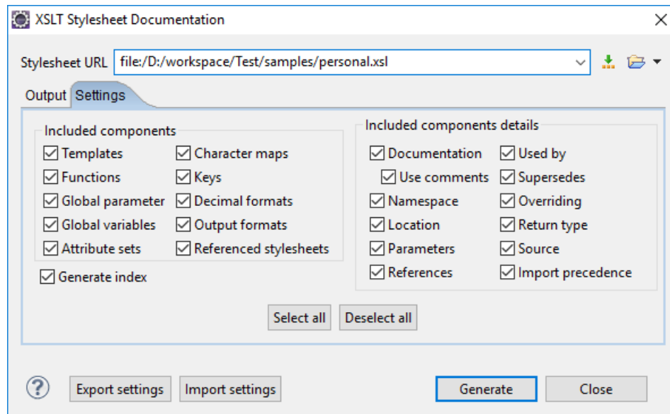
Figure 209: Settings Tab of the XSLT Stylesheet Documentation Dialog Box
