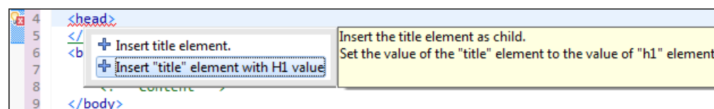
Figure 161: Example of a Schematron Quick Fix
