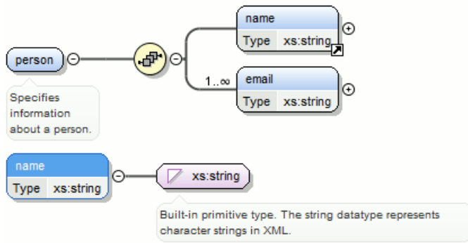
Figure 219: Extracting a Global Element on a name Element
