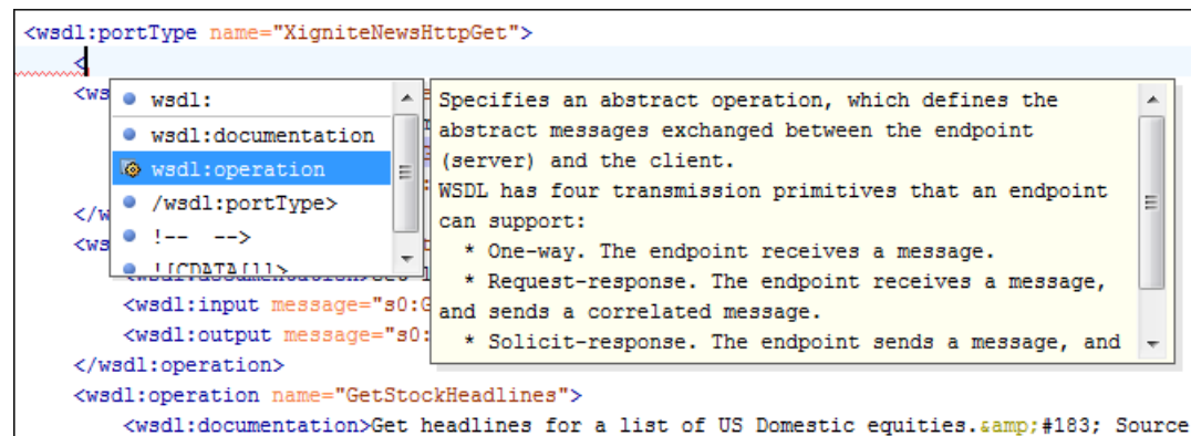
Figure 298: WSDL Content Completion Assistant
