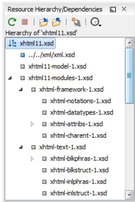
Figure 264: Resource Hierarchy/Dependencies View - Hierarchy for xhtml11.xsd
