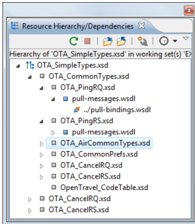
Figure 302: Resource Hierarchy/Dependencies View
