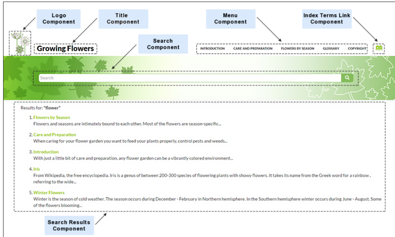
Figure 378: Examples of Search Results Page Components
