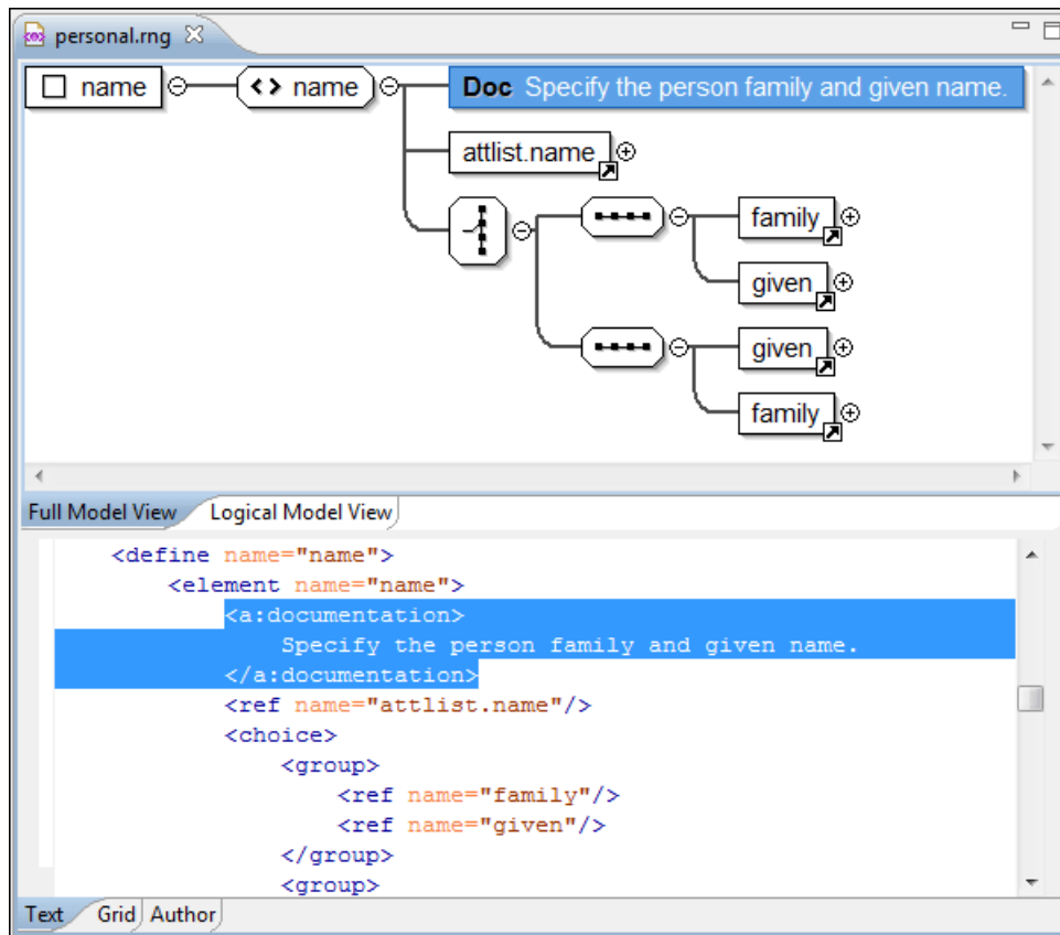
Figure 316: Relax NG Schema Editor - Full Model View
