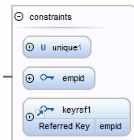
Figure 112: Constraints Construct
