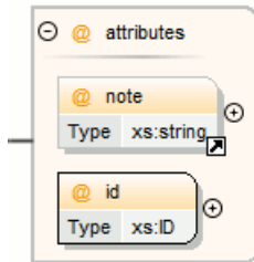
Figure 111: Attributes Construct
