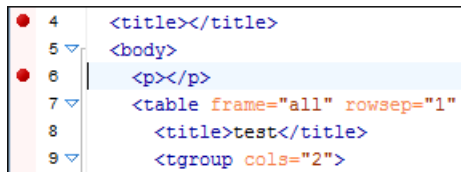
Figure 440: Example: Breakpoints
