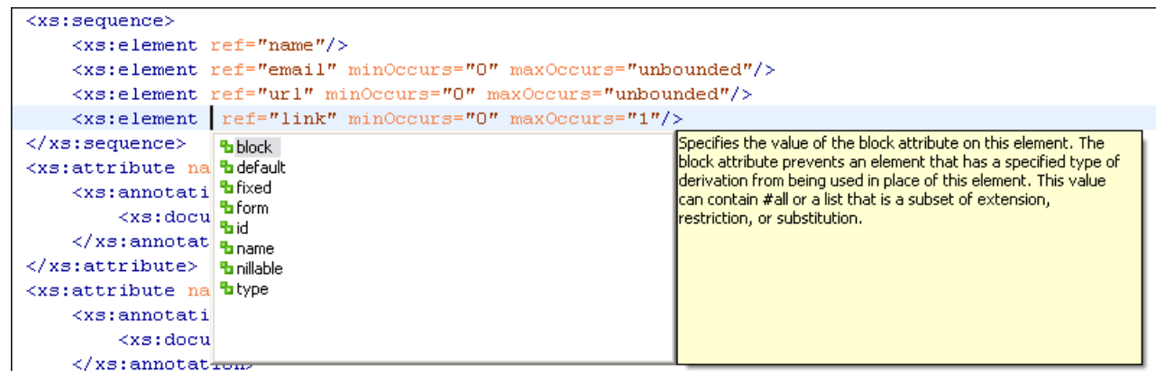
Figure 136: Content Completion Assistant
