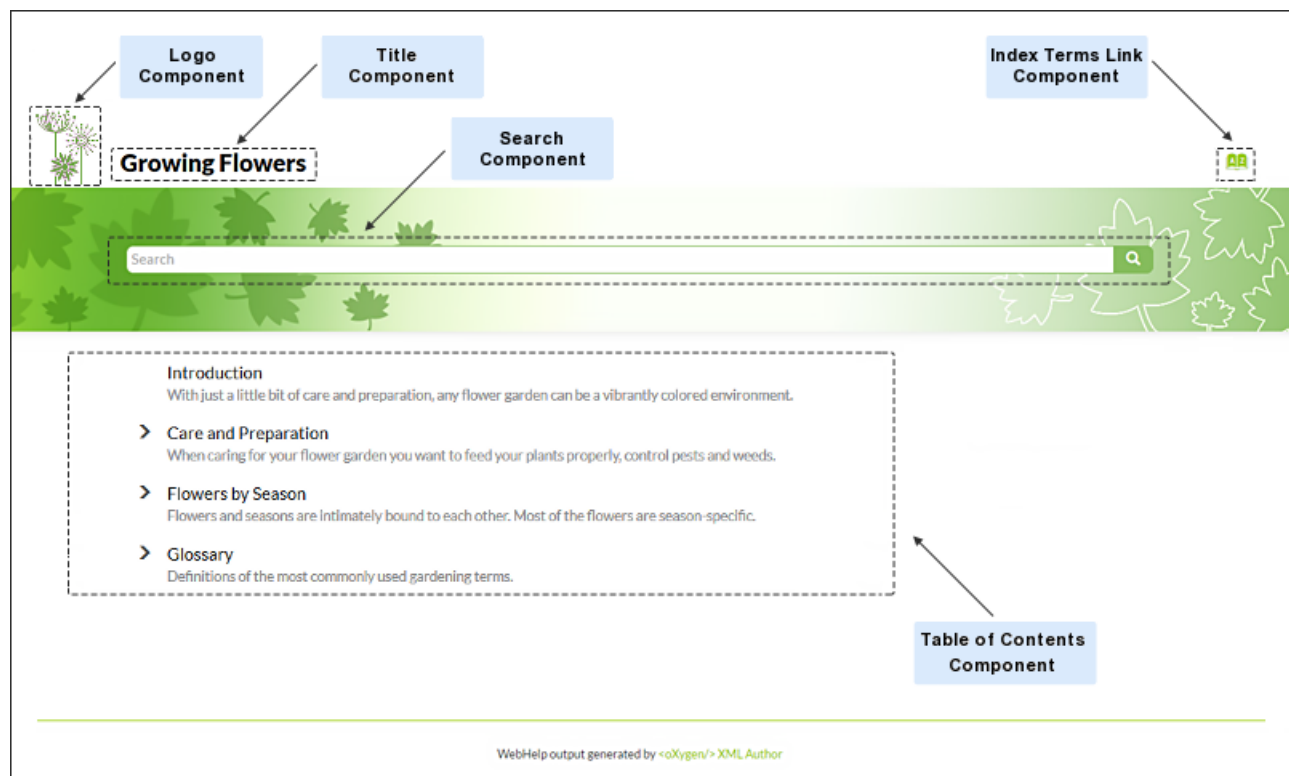
Figure 376: Examples of Main Page Components for a Tree Style of Layout
