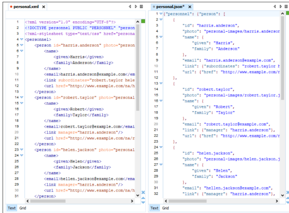
Figure 336: Example: XML to JSON Operation Result
