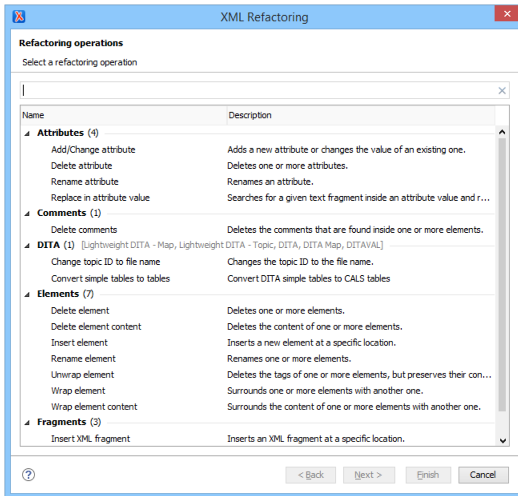
Figure 173: XML Refactoring Wizard
