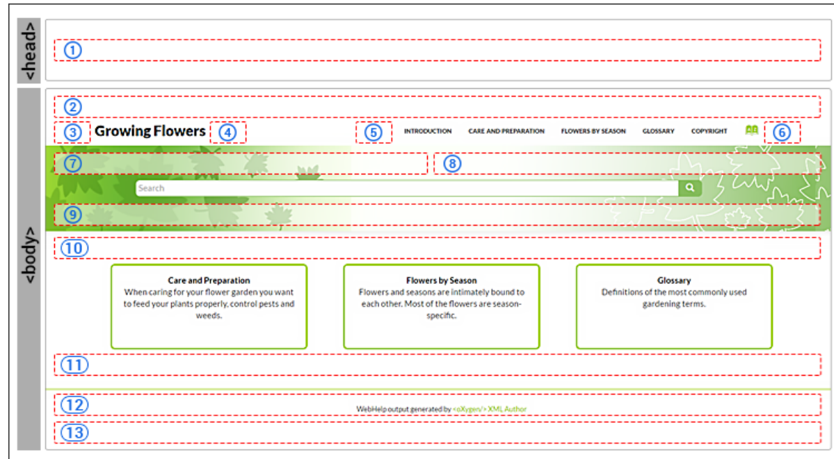
Figure 380: Predefined Placeholders Diagram
