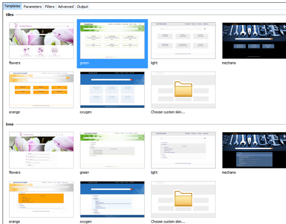
Figure 360: Templates Tab
