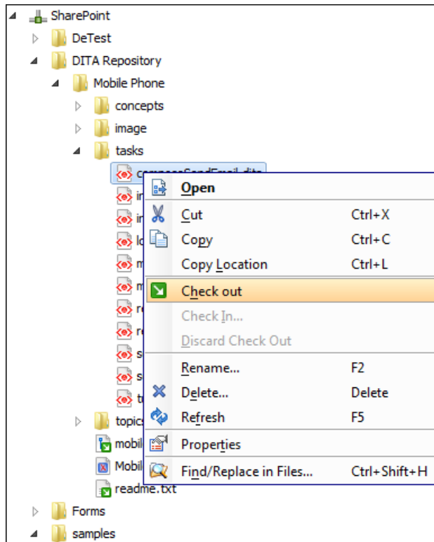
Figure 421: SharePoint Connection
