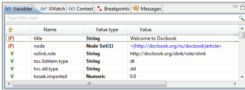
Figure 438: Variables View
