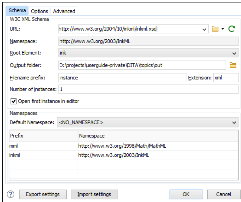
Figure 269: Generate Sample XML Files Dialog Box (Schema Tab)
