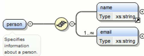
Figure 74: Extracting a Global Element
