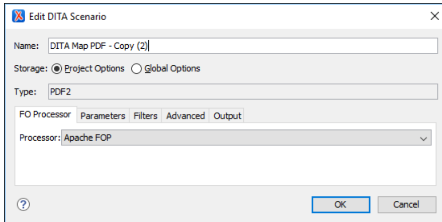
Figure 365: Edit Scenarios Configuration Dialog Box
