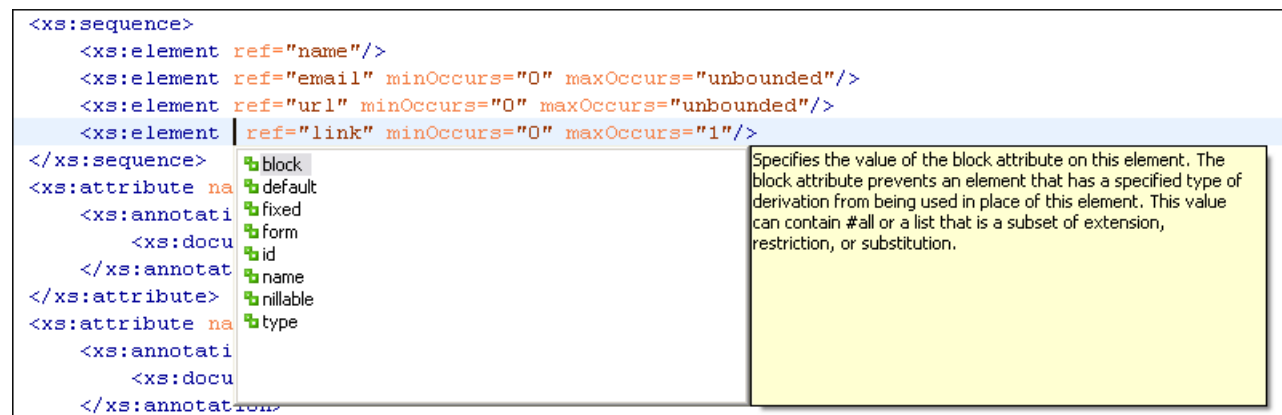
Figure 37: Content Completion Assistant
