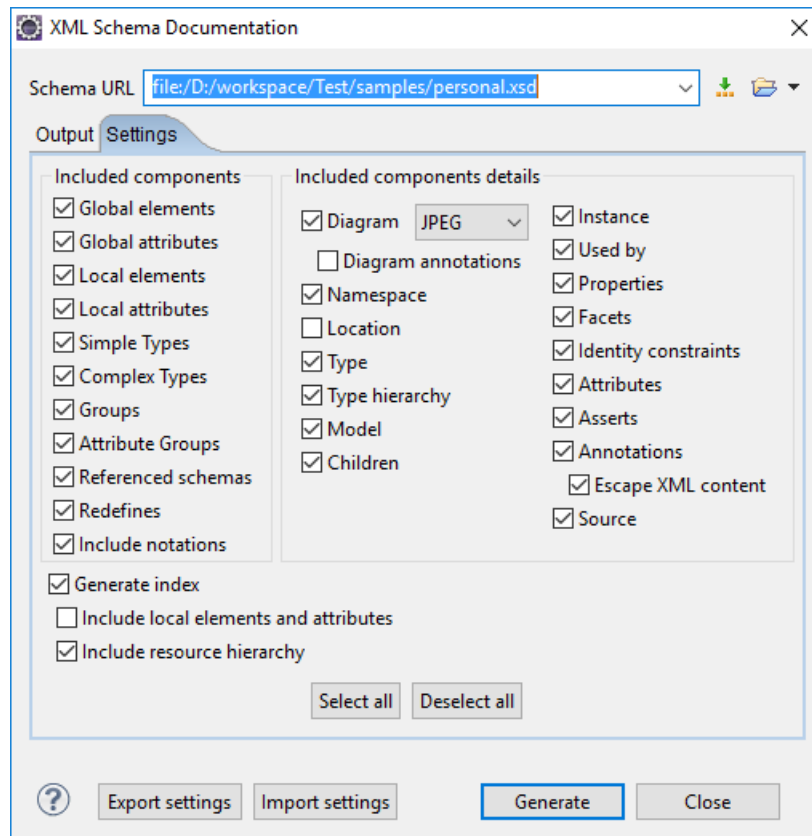
Figure 273: Settings Tab of the XML Schema Documentation Dialog Box
