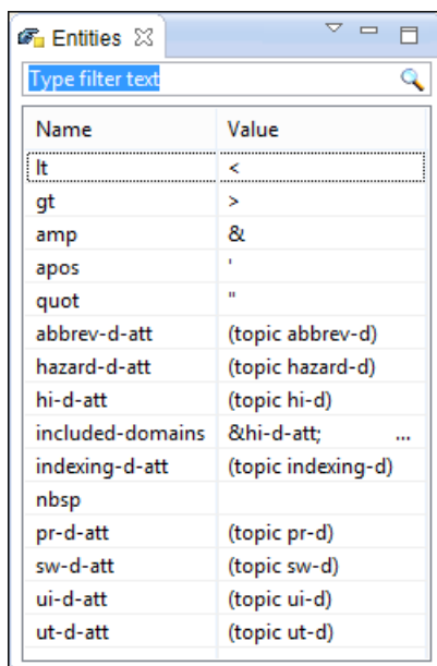
Figure 143: Entities View
