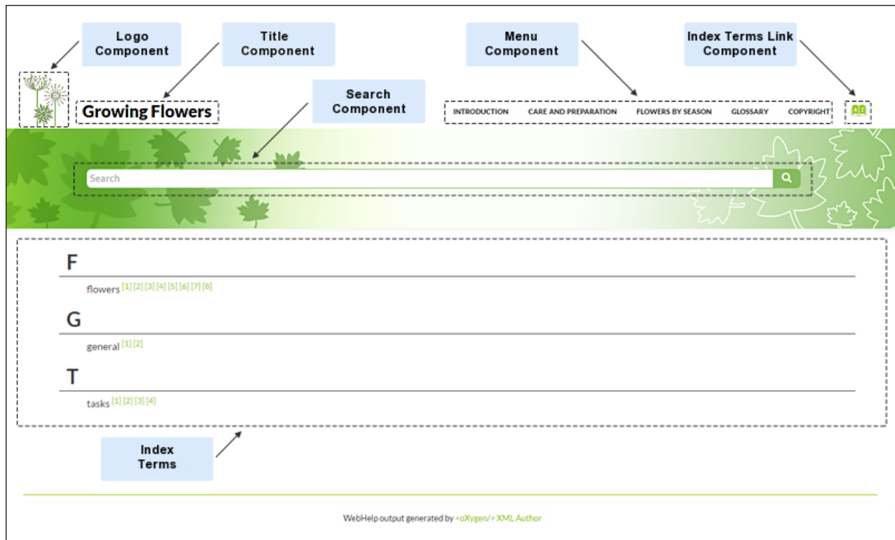
Figure 379: Examples of Index Terms Page Components
