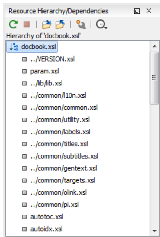
Figure 237: Resource Hierarchy/Dependencies View - Hierarchy for docbook . xsl
