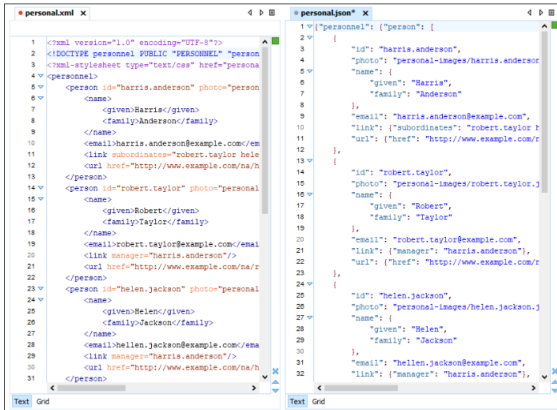
Figure 515: Example: XML to JSON Operation Result
