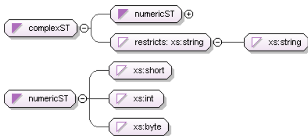
Figure 101: Extracting a Global Simple Type on a union Component
