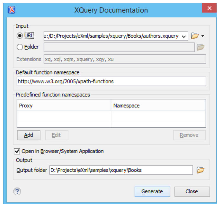
Figure 522: XQuery Documentation Dialog Box
