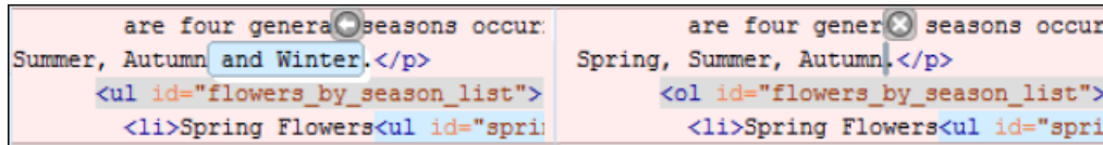
Figure 312: Second Level Diff Comparison
