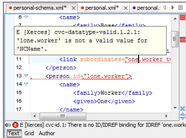
Figure 109: Presenting Validation Errors in Text Mode
