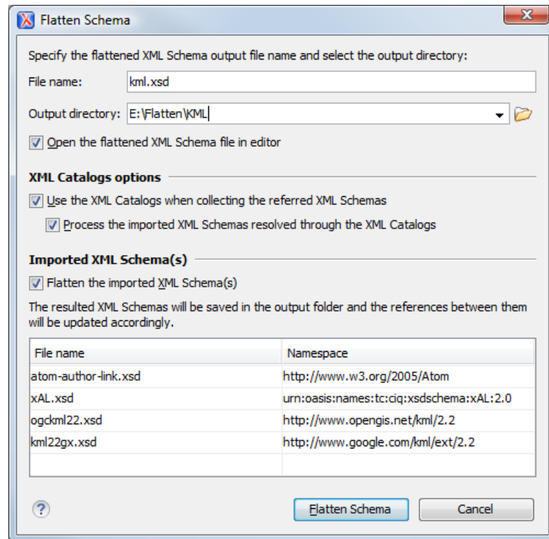
Figure 434: Flatten Schema Dialog Box
