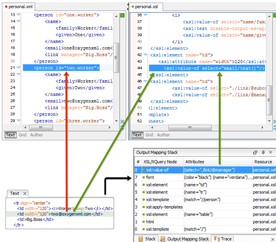
Figure 419: Text Output to Source Mapping
