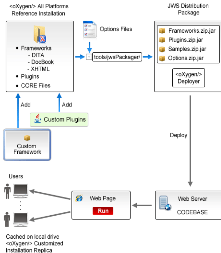
Figure 2: Java Web Start Deployment Procedure
