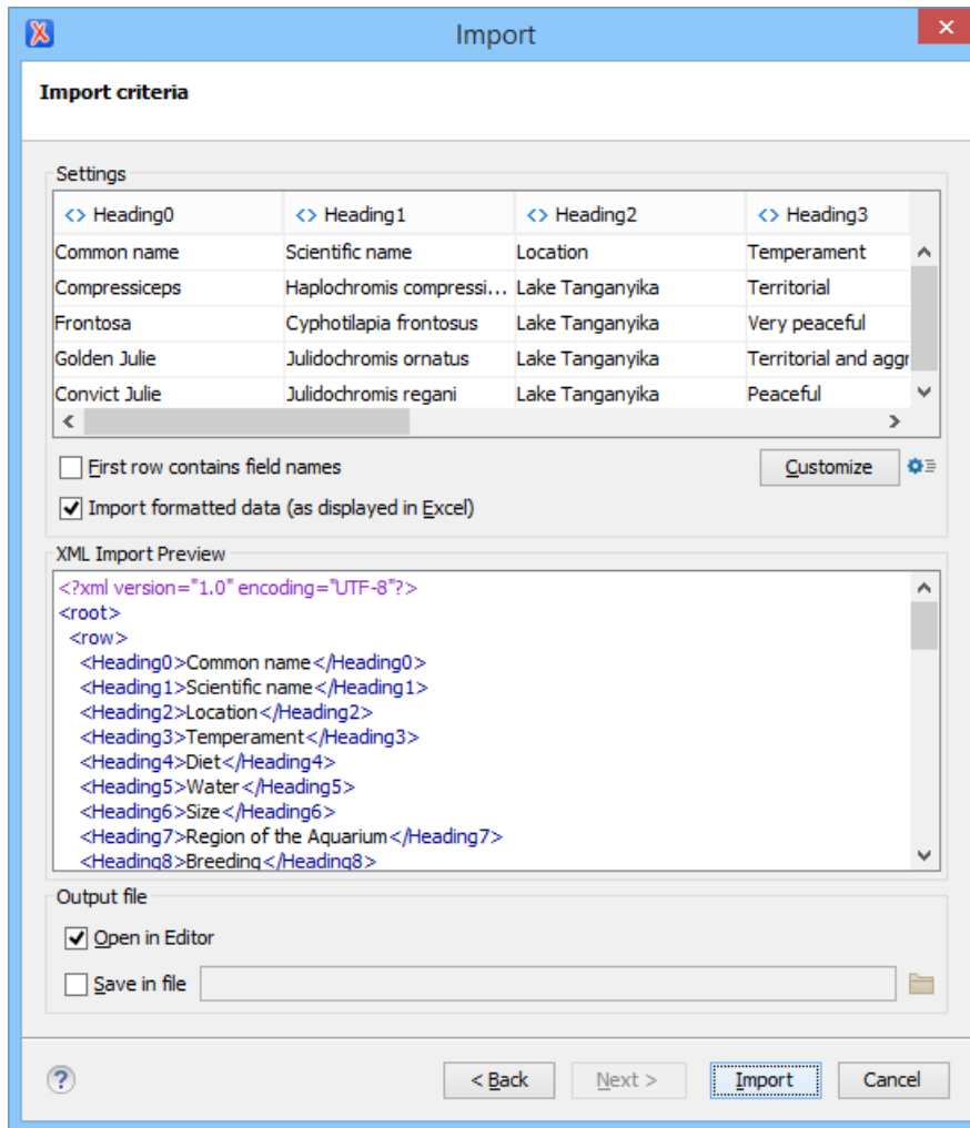
Figure 400: Import Criteria Dialog Box
