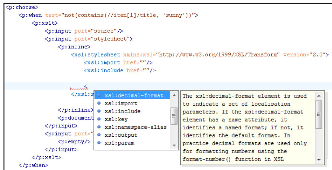
Figure 287: XProc Content Completion
