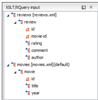
Figure 156: XQuery Input View
