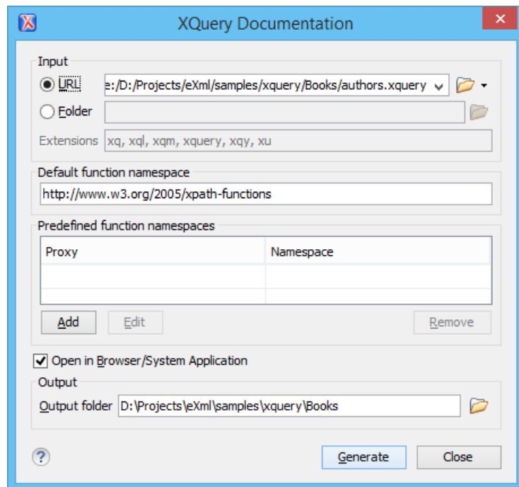
Figure 442: XQuery Documentation Dialog Box
