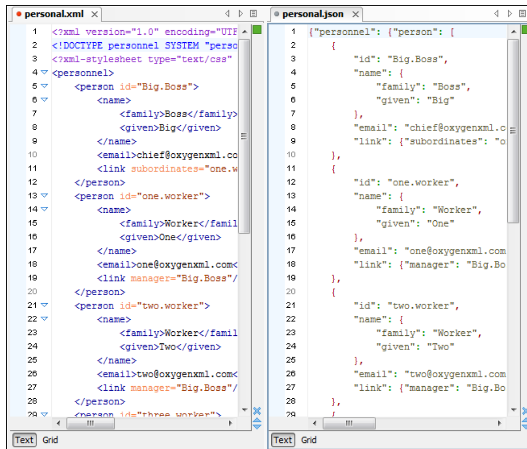
Figure 436: Example: XML to JSON Operation Result
