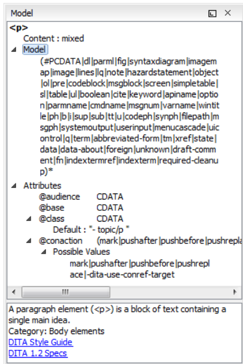
Figure 54: Model View
