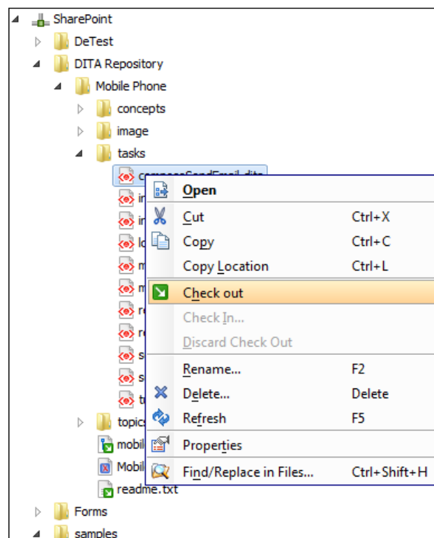
Figure 395: SharePoint Connection
