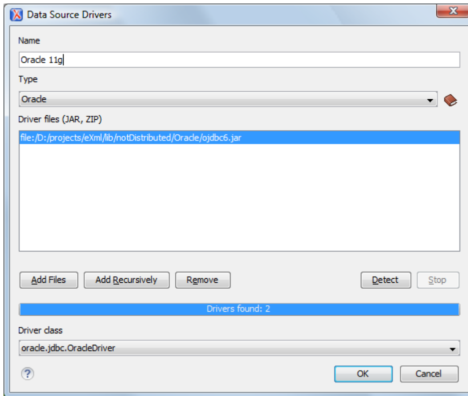
Figure 25: Data Sources Drivers Dialog Box
