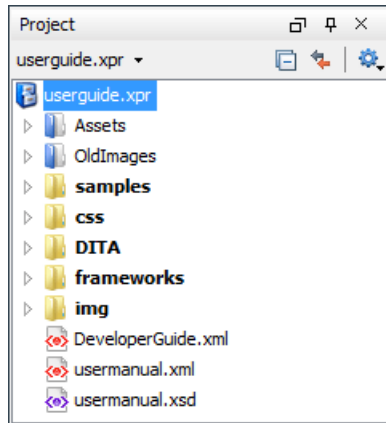
Figure 85: Project View
