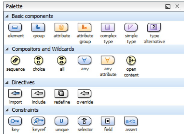
Figure 220: Palette View
