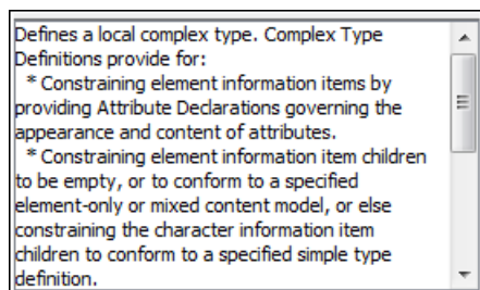
Figure 98: Annotation panel
