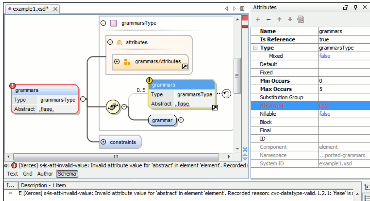
Figure 219: XML Schema Validation
