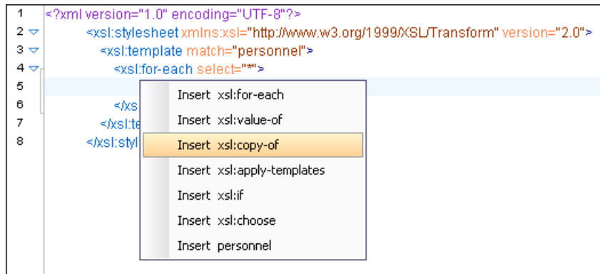
Figure 154: XSLT Input Drag and Drop Pop-up Menu
