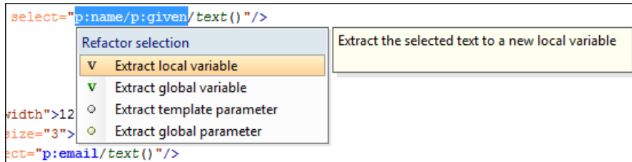
Figure 169: XSLT Quick Assist Support - Refactoring Actions
