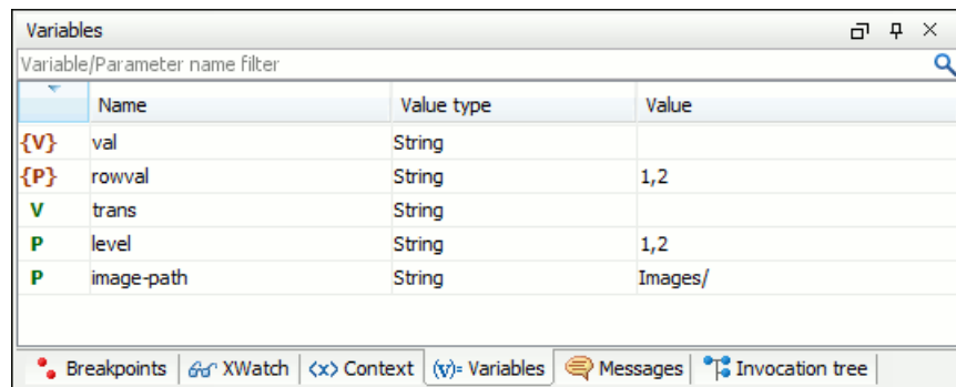
Figure 416: Variables View
