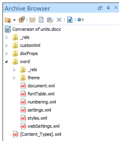
Figure 365: Archive Browser
