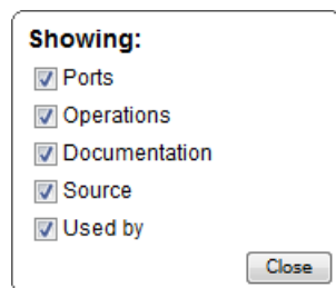
Figure 260: Showing Options
