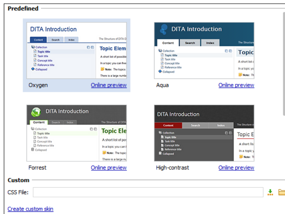
Figure 324: Skins Tab
