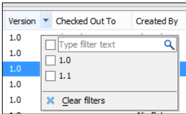
Figure 81: Column Filter
