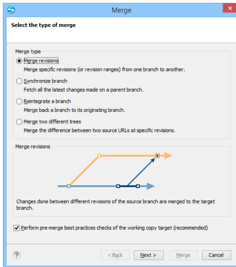
Figure 481: Merge Wizard
