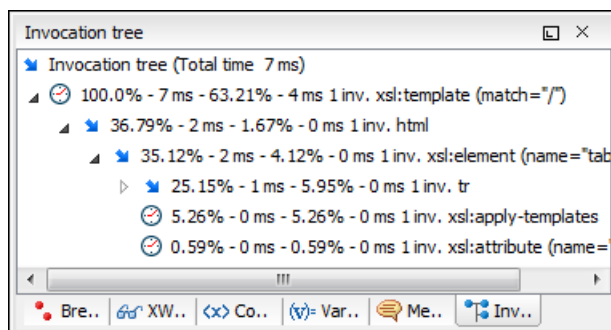
Figure 421: Invocation Tree View
