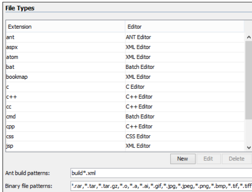
Figure 38: File Types Preferences Page
