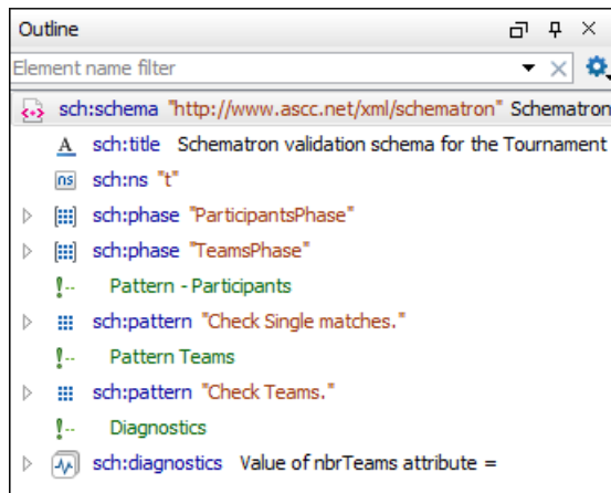
Figure 289: Schematron Outline View
