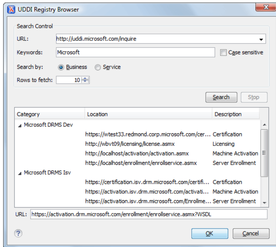
Figure 263: UDDI Registry Browser Dialog Box
