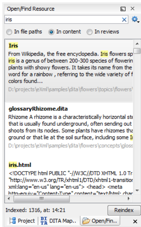
Figure 51: Open/Find Resource View
