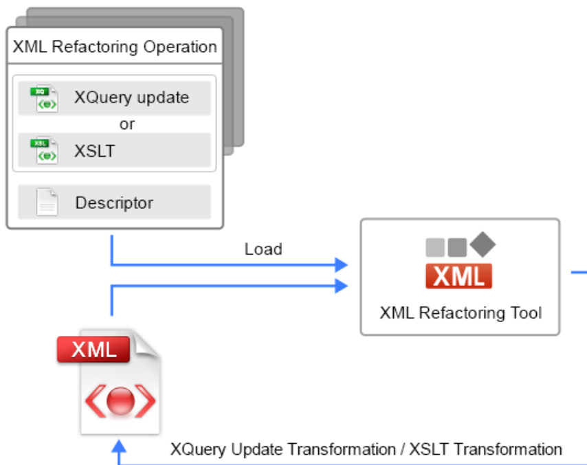
Figure 138: Diagram of an XML Refactoring Operation
