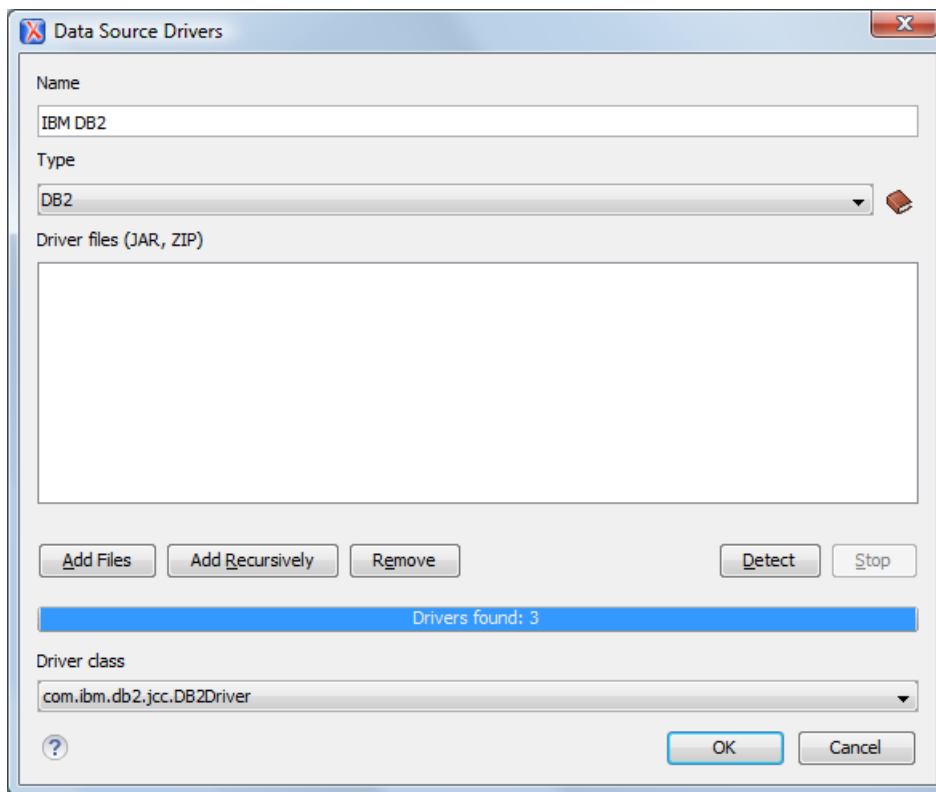
Figure 372: Data Source Drivers Configuration Dialog Box
