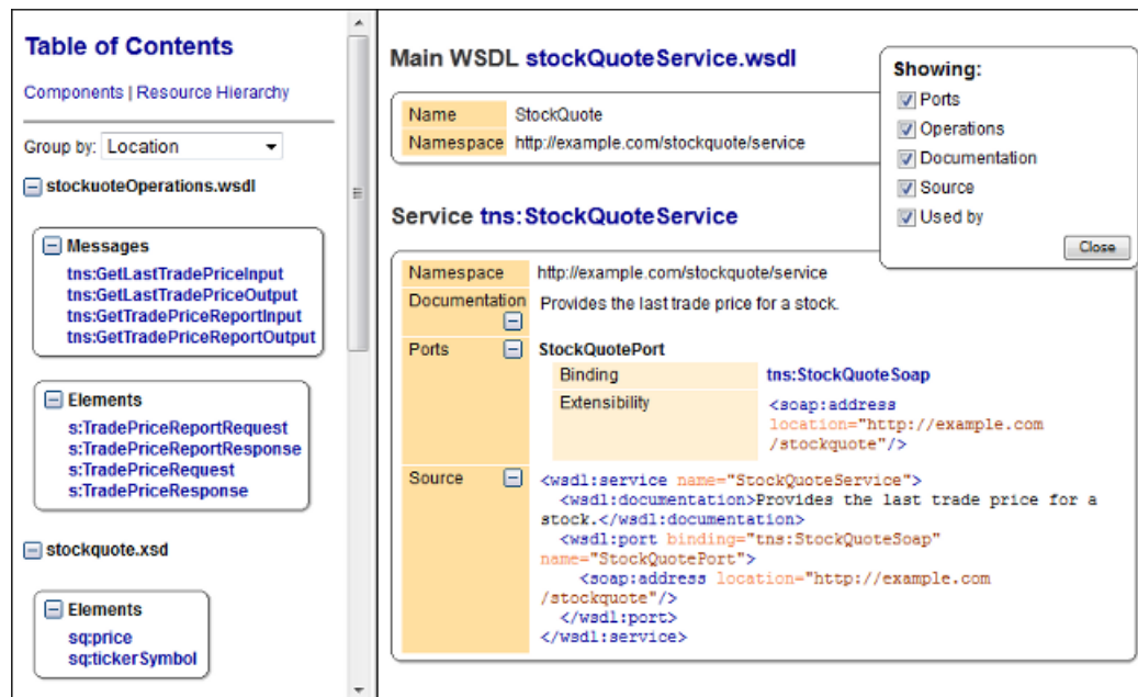
Figure 259: WSDL Documentation in HTML Format
