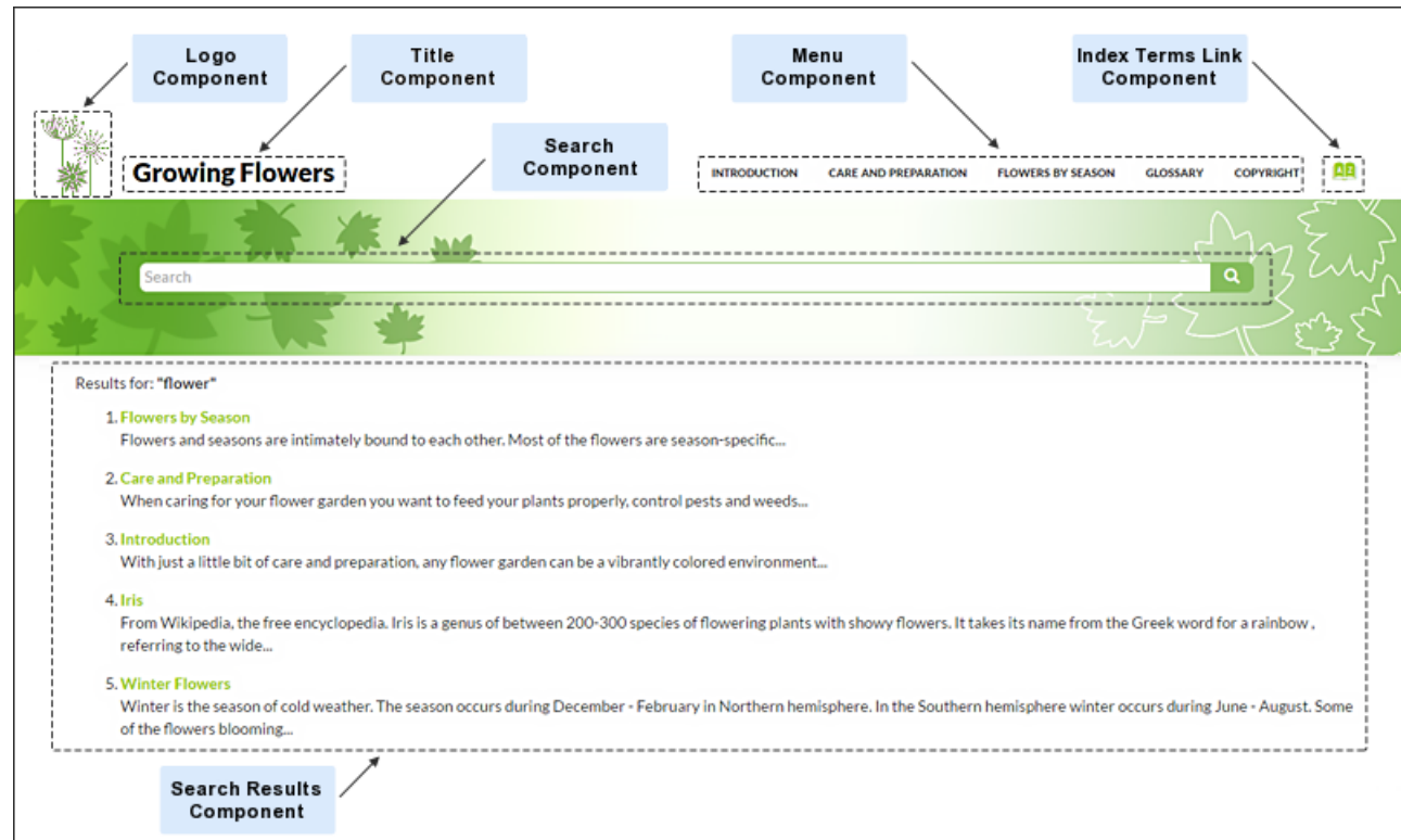
Figure 340: Example: Search Results Page Components
