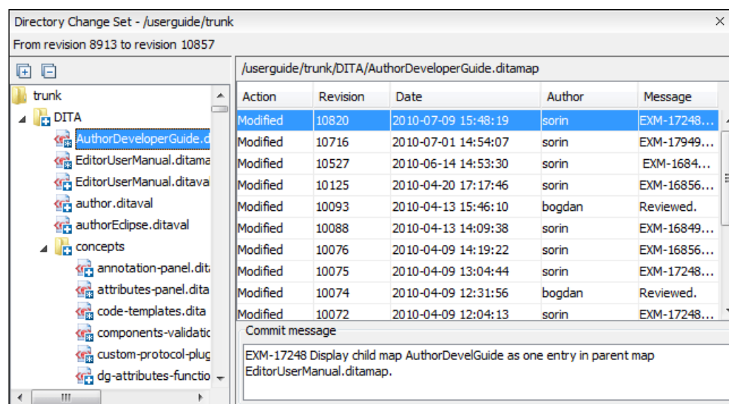
Figure 507: Directory Change Set View
