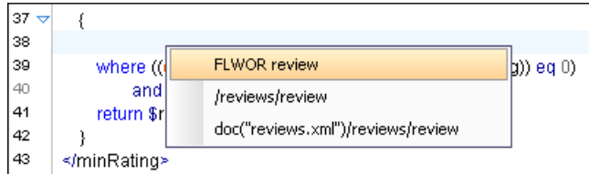
Figure 360: XQuery Input Drag and Drop Pop-up Menu
