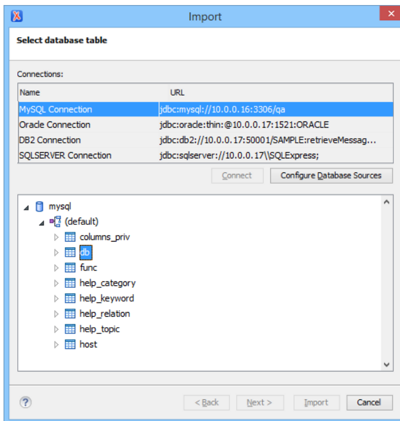
Figure 401: Select Database Table Dialog Box
