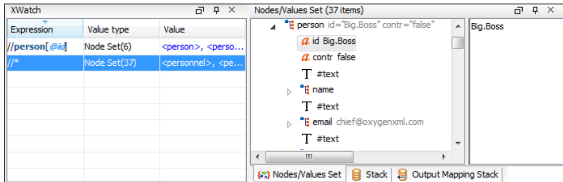
Figure 408: XPath Watch View
