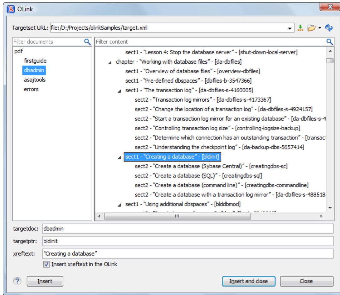
Figure 322: Insert OLink Dialog Box
