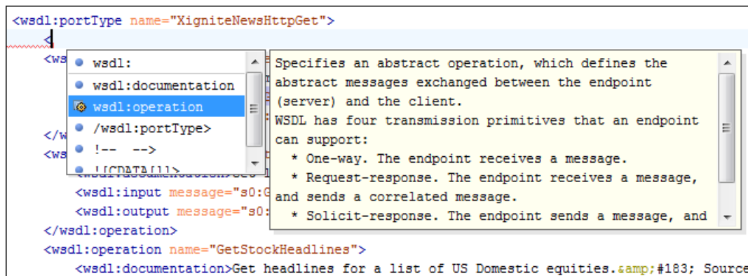
Figure 248: WSDL Content Completion Assistant
