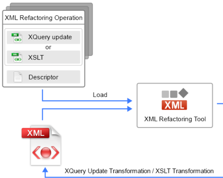
Figure 427: Diagram of an XML Refactoring Operation
