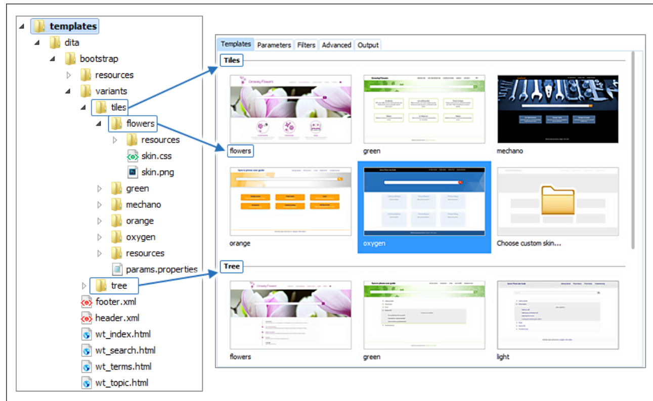
Figure 336: Templates Directory Structure
