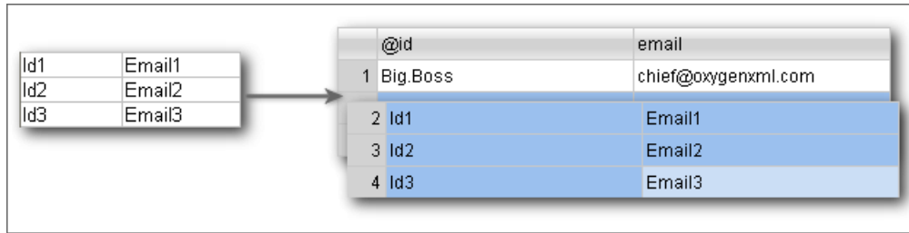
Figure 107: Pasting Tab-Separated Values into Grid
