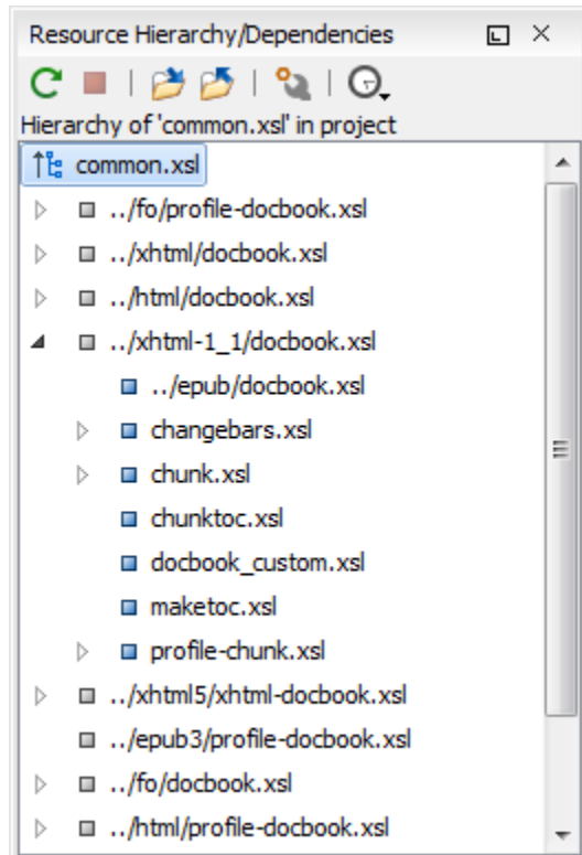
Figure 160: Resource Hierarchy/Dependencies View - Dependencies for common.xml
