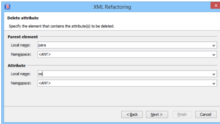
Figure 136: XML Refactoring 2nd Wizard Page (Delete Attribute Operation)
