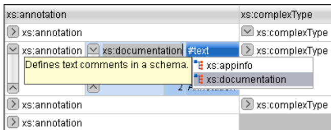
Figure 108: Content Completion in Grid Editing Mode
