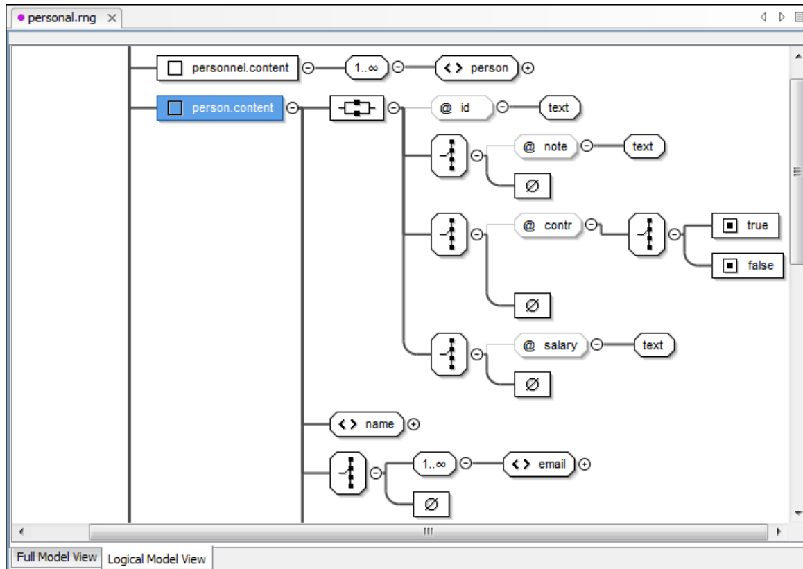
Figure 268: Logical Model View for a Relax NG Schema
