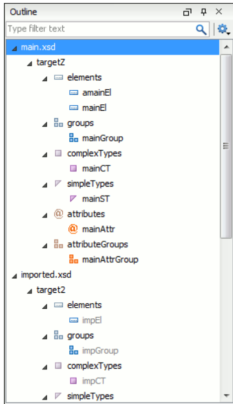
Figure 69: Outline View for XML Schema
