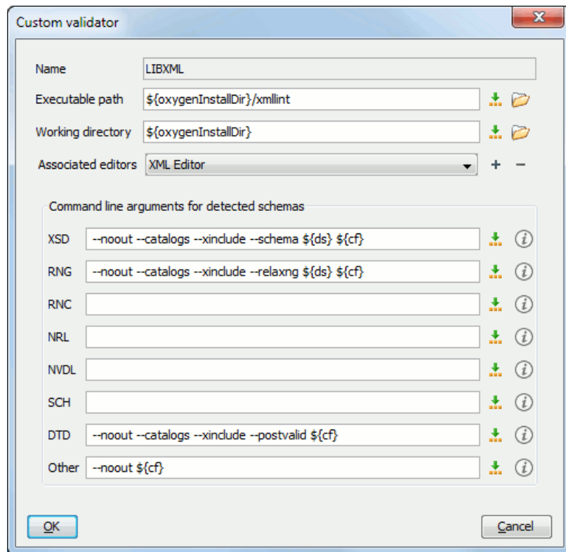
Figure 15: Custom Validator Dialog Box
