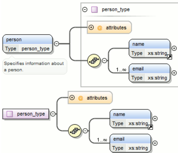
Figure 188: Extracting a Global Complex Type on a person Element
