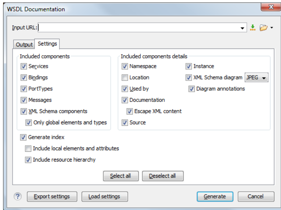
Figure 444: Settings Tab of the WSDL Documentation Dialog Box
