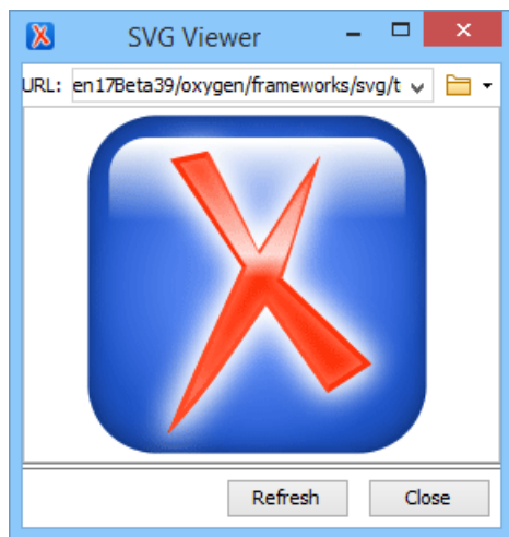
Figure 298: SVG Viewer
