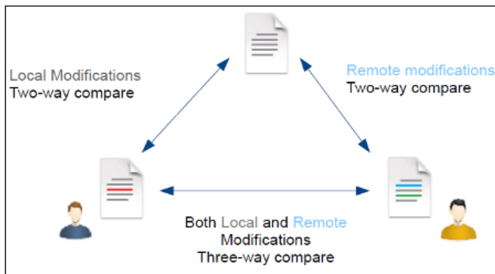
Figure 310: Three-Way Comparison
