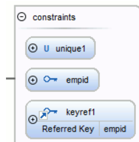
Figure 217: Constraints Construct
