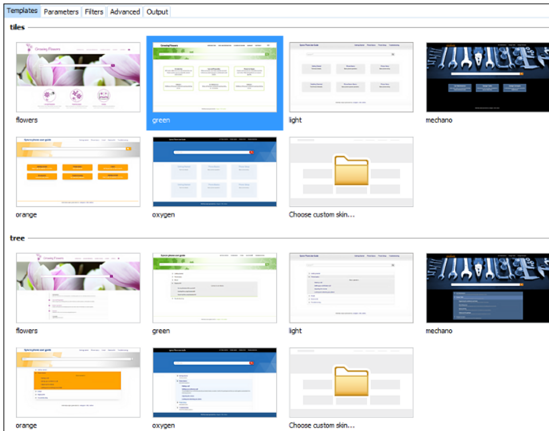
Figure 325: Templates Tab
