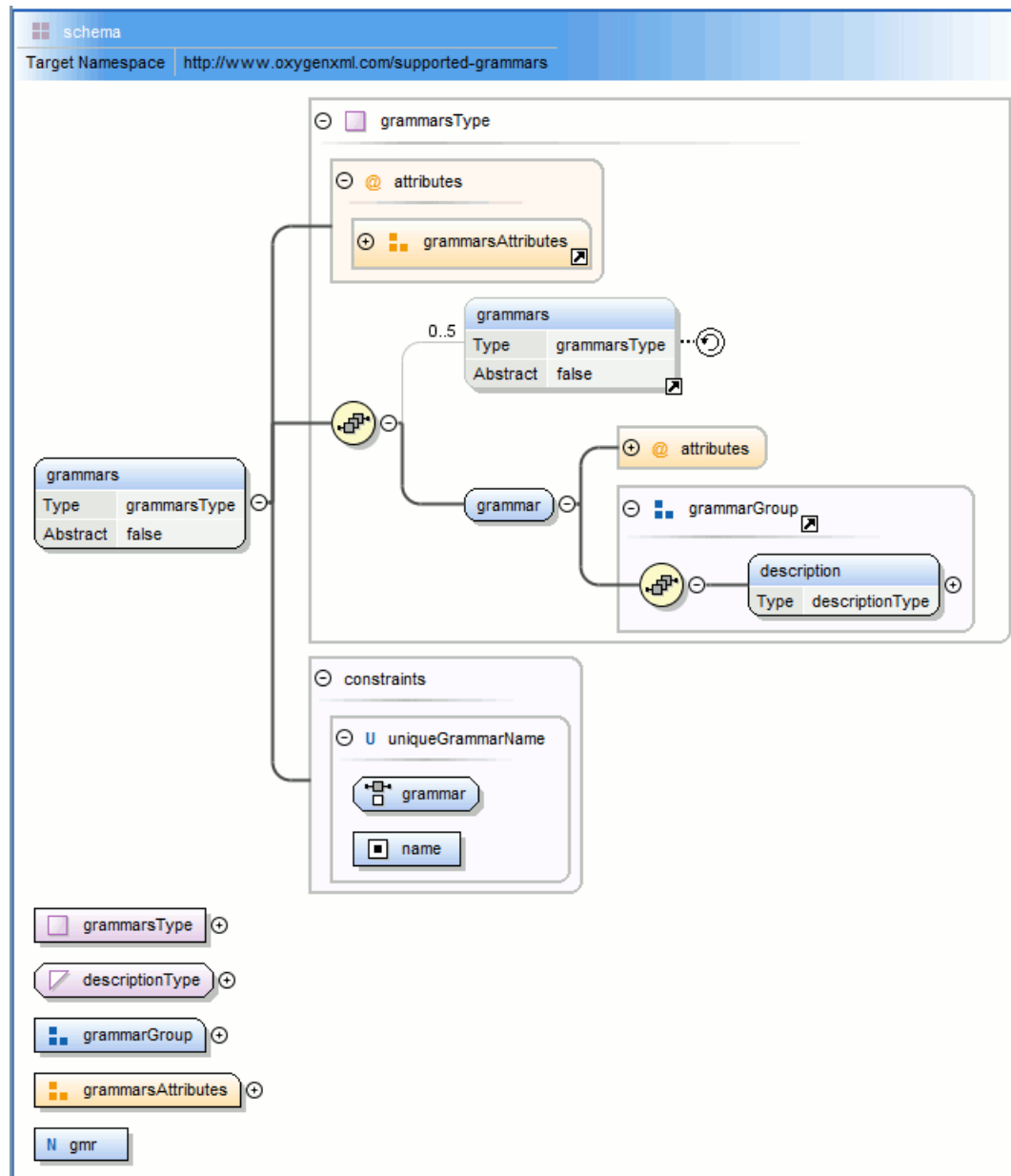
Figure 177: XML Schema Diagram
