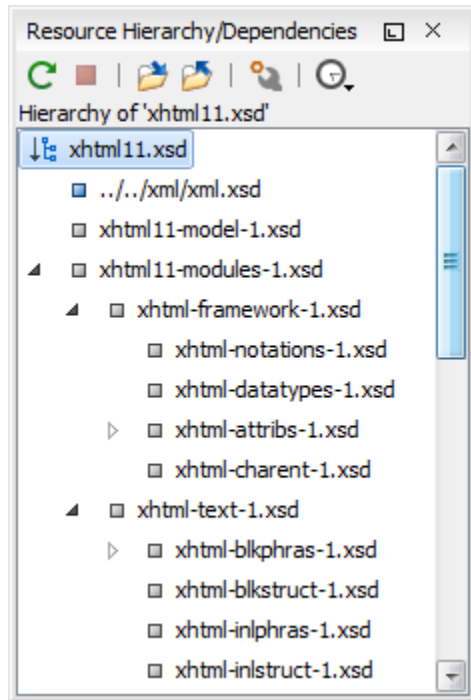
Figure 225: Resource Hierarchy/Dependencies View - Hierarchy for xhtml11.xsd
