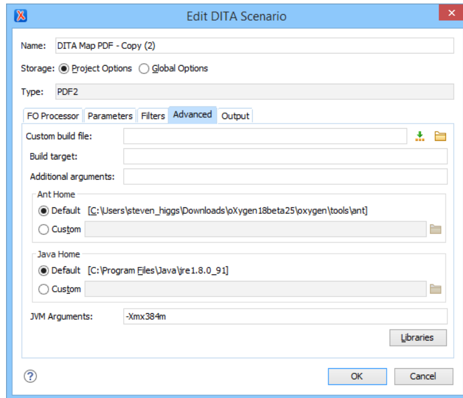
Figure 327: Advanced Settings Tab
