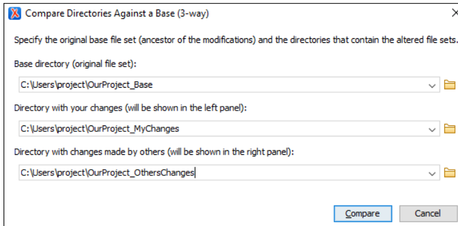
Figure 318: Compare Directories Against a Base File Set Chooser
