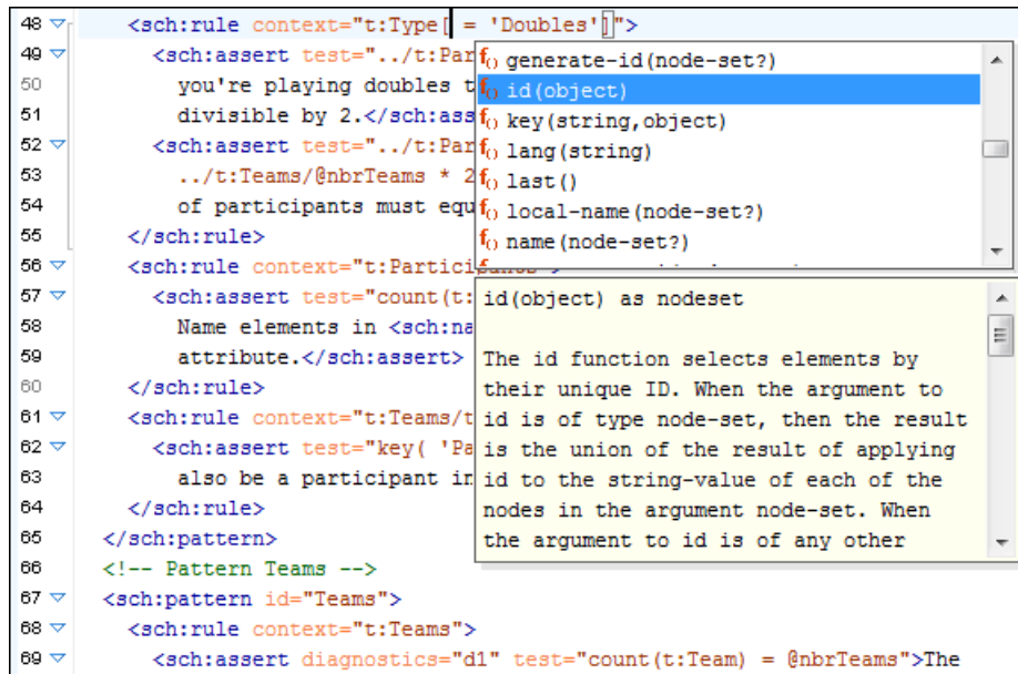
Figure 288: XSLT Extension Functions in Schematron Schema Content Completion
