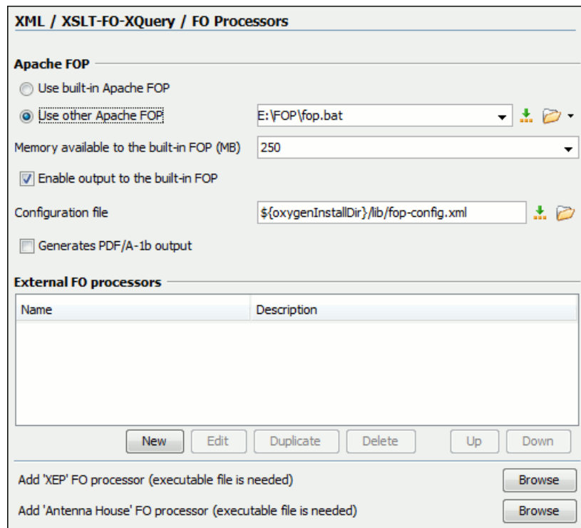
Figure 20: FO Processors Preferences Page
