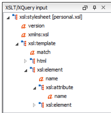
Figure 143: XSLT Input View
