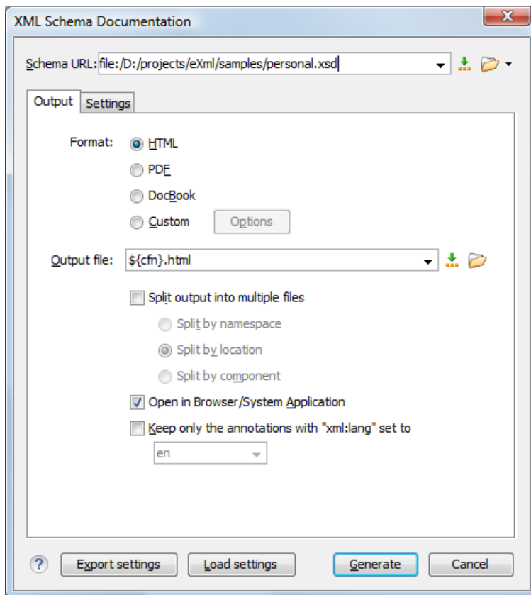
Figure 405: XML Schema Documentation Dialog Box
