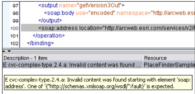
Figure 234: Validating a WSDL file
