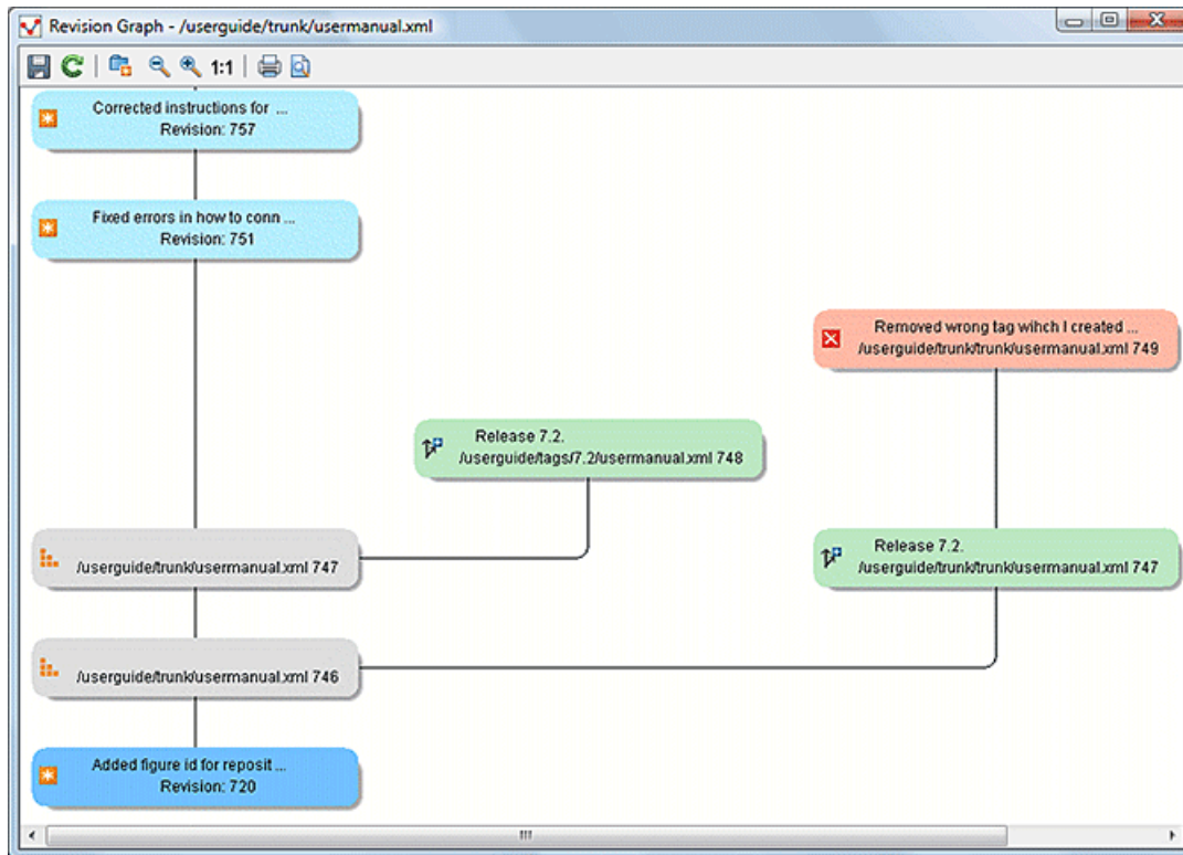
Figure 477: Revision Graph of a File Resource
