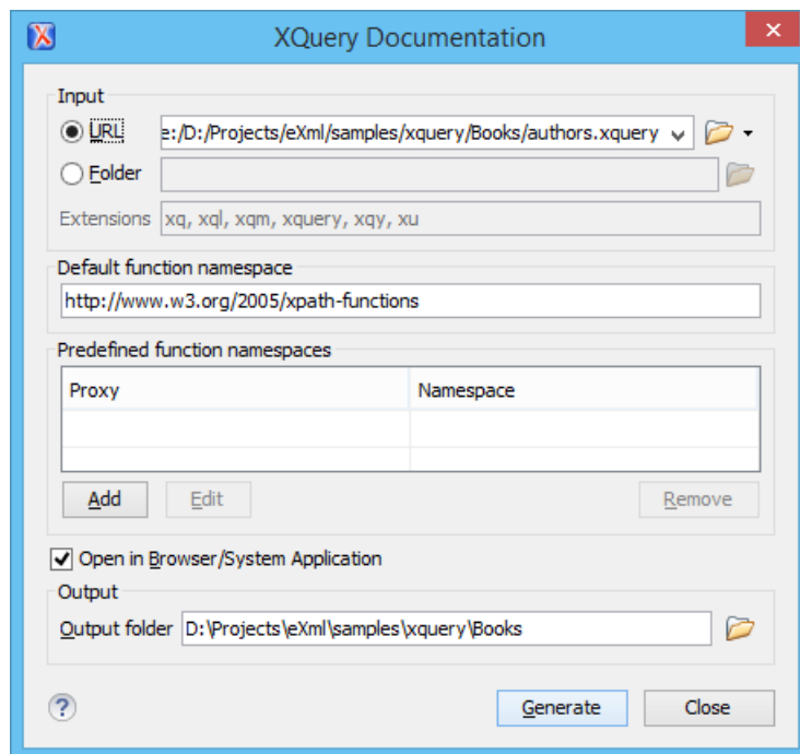
Figure 409: XQuery Documentation Dialog Box
