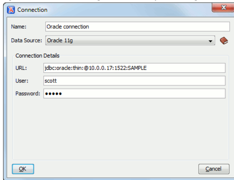
Figure 25: Connection Dialog Box
