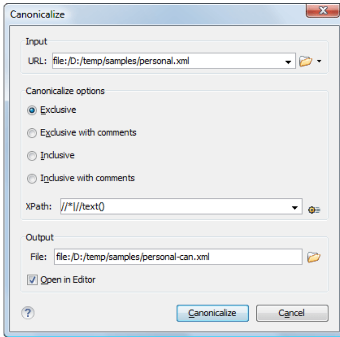
Figure 412: Canonicalization Settings Dialog Box
