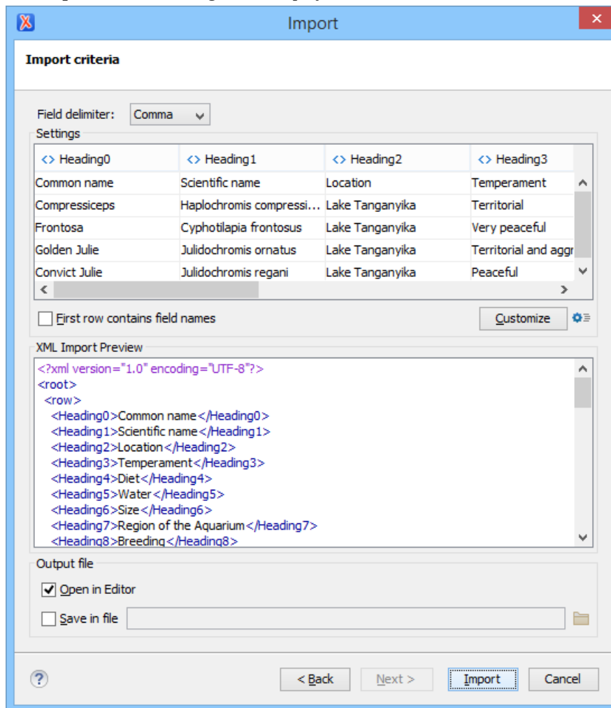
Figure 364: Import Criteria Dialog Box
