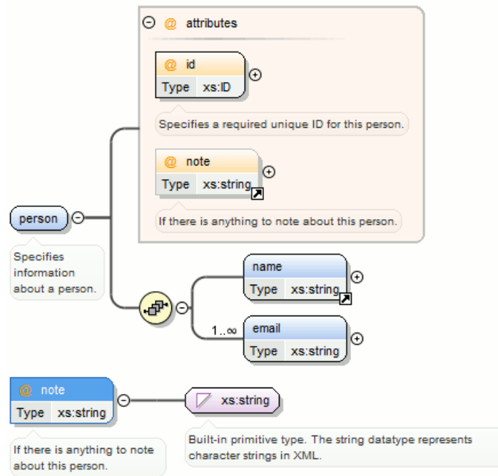
Figure 169: Extracting a Global Attribute on a note Attribute
