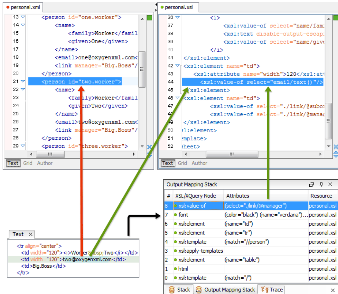
Figure 384: Text Output to Source Mapping
