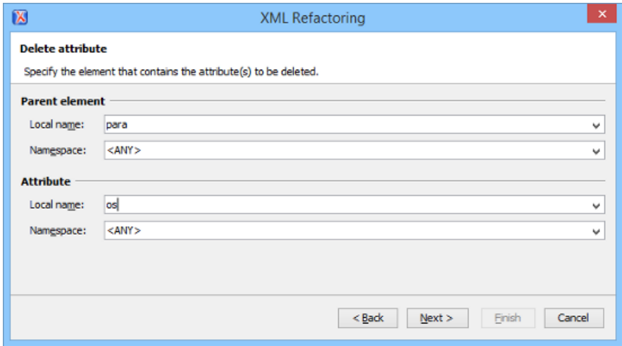
Figure 392: XML Refactoring 2nd Wizard Page (Delete Attribute Operation)
