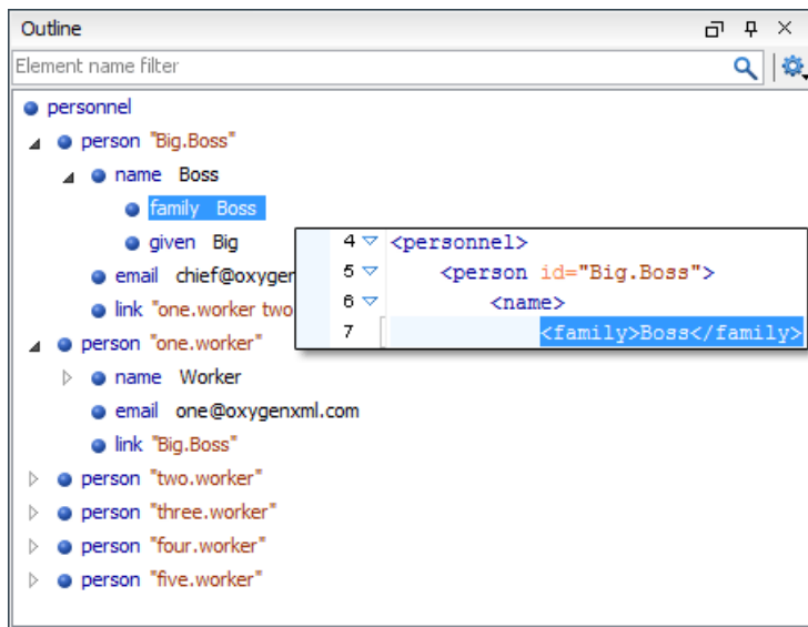
Figure 49: Outline View in Text Mode
