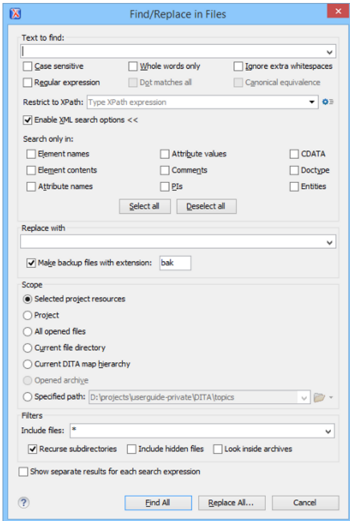
Figure 113: Find / Replace in Files Dialog Box
