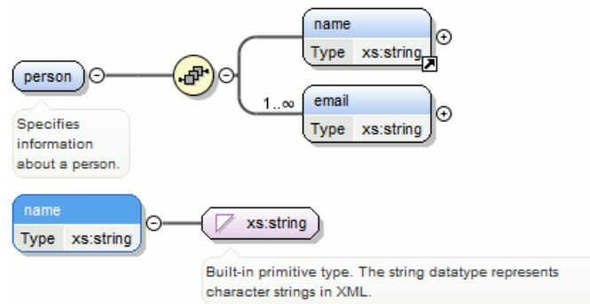
Figure 167: Extracting a Global Element on a name Element
