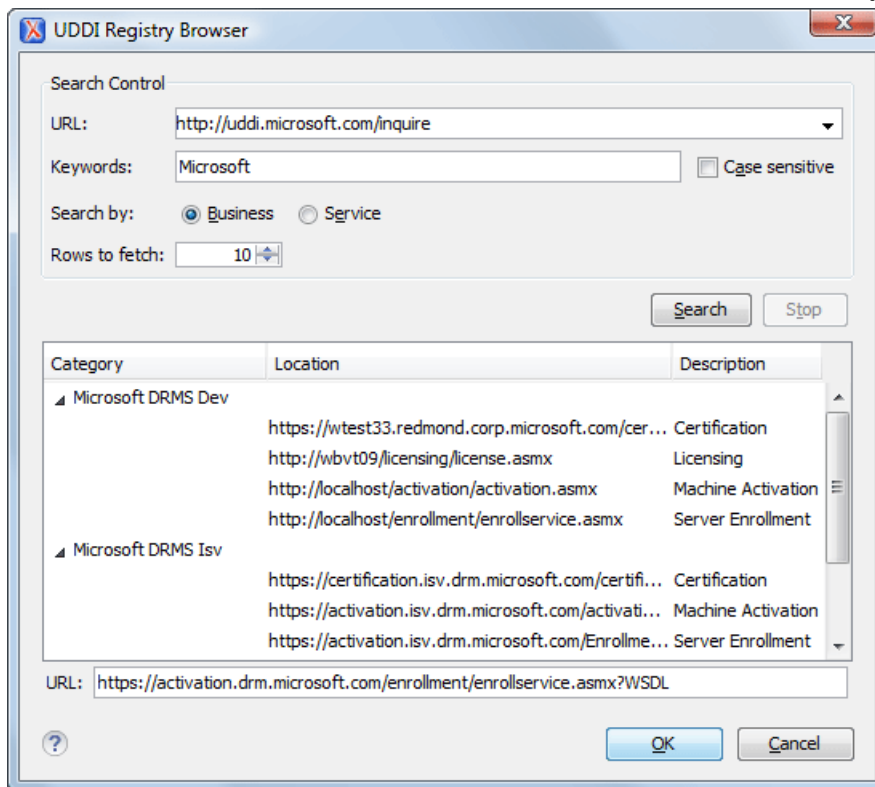
Figure 250: UDDI Registry Browser Dialog Box
