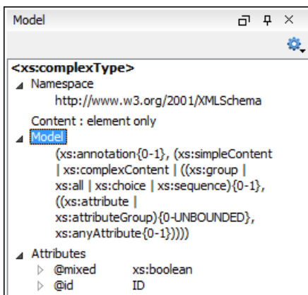
Figure 94: Element Structure Panel
