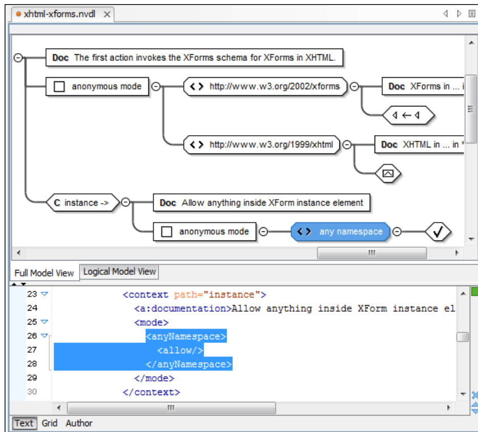
Figure 262: NVDL Schema Editor - Full Model View
