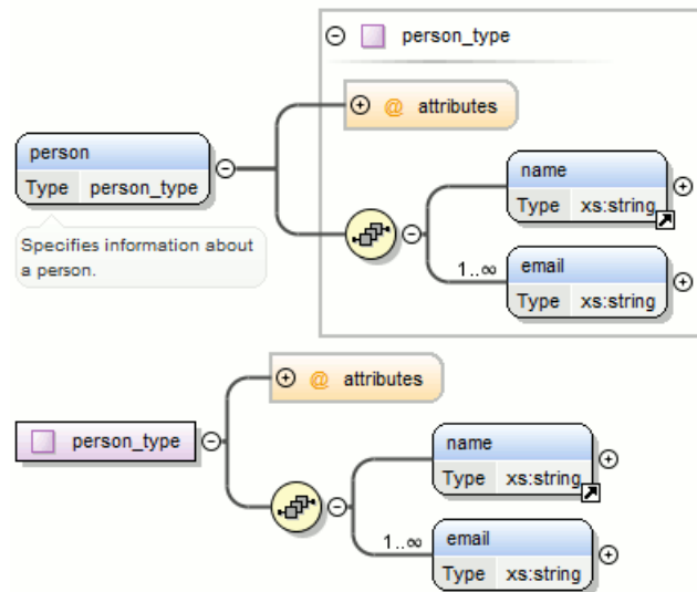
Figure 175: Extracting a Global Complex Type on a person Element
