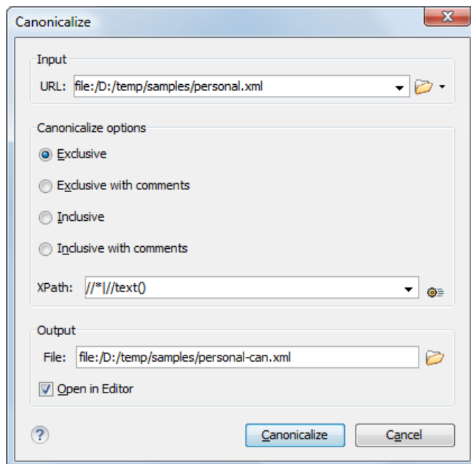
Figure 288: Canonicalization Settings Dialog Box
