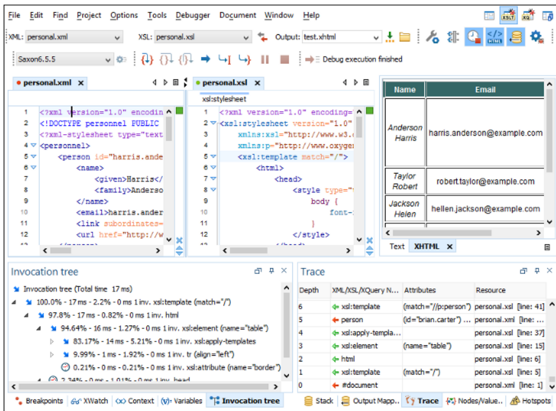
Figure 368: Debugger Mode Interface
