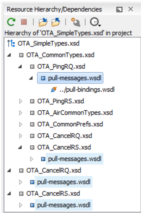
Figure 239: Resource Hierarchy/Dependencies View
