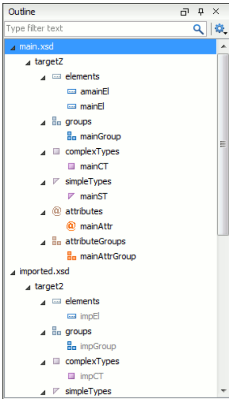
Figure 67: Outline View for XML Schema
