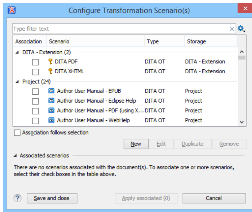
Figure 307: Configure Transformation Scenario(s) Dialog Box
