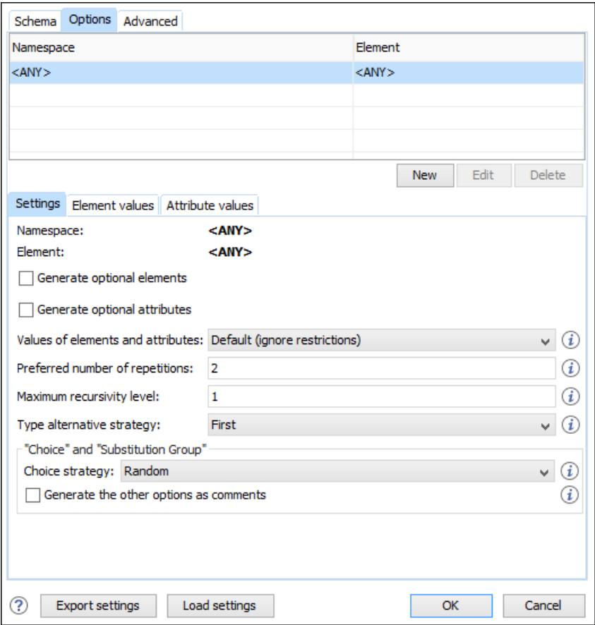
Figure 398: Generate Sample XML Files Dialog Box (Options Tab)
