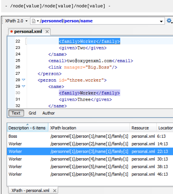
Figure 322: XPath Results Highlighted in Editor Panel with Character Precision
