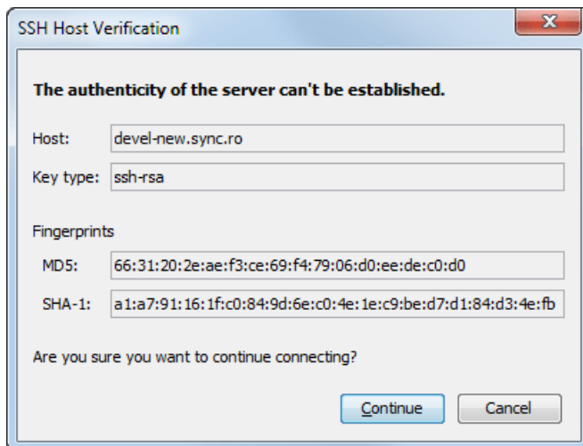
Figure 433: SSH server name and key fingerprint
