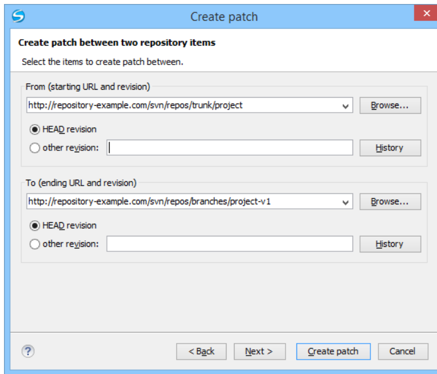
Figure 454: Create Patch Wizard - Step 2
