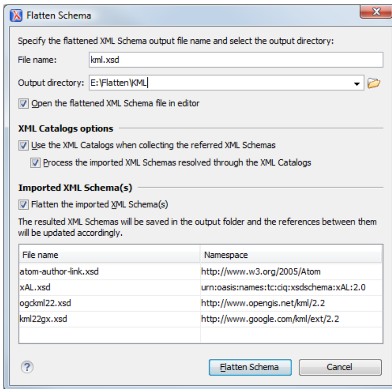
Figure 401: Flatten Schema Dialog Box
