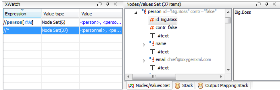
Figure 373: XPath Watch View
