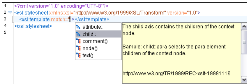
Figure 134: Content Completion in the match Attribute
