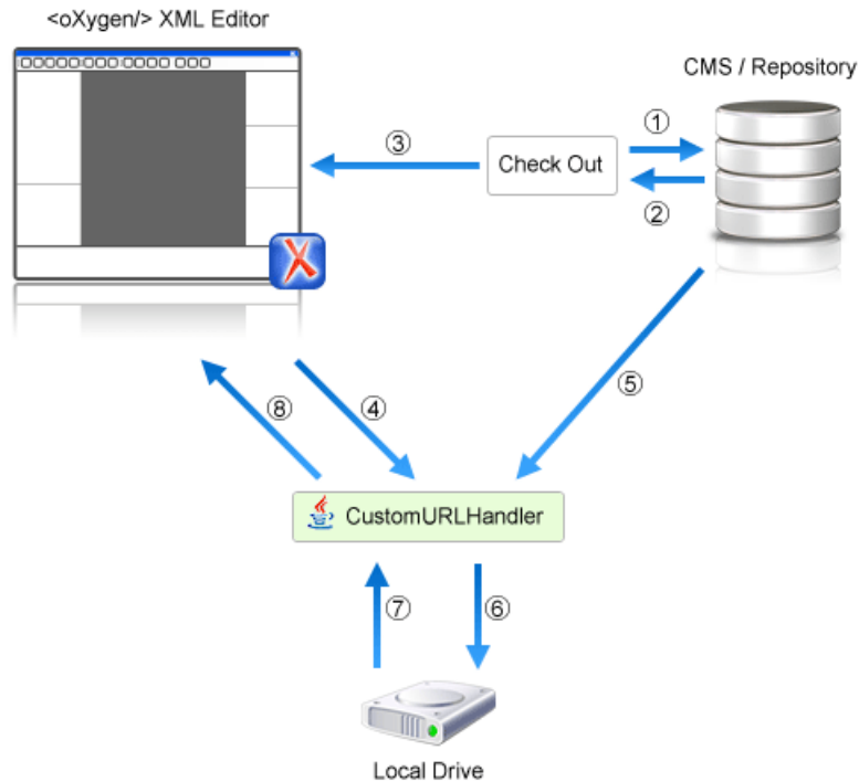
Figure 390: Check Out Process Diagram
