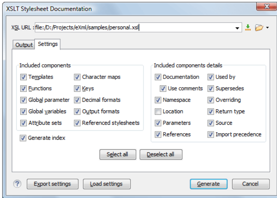
Figure 150: Settings Tab of the XSLT Stylesheet Documentation Dialog Box
