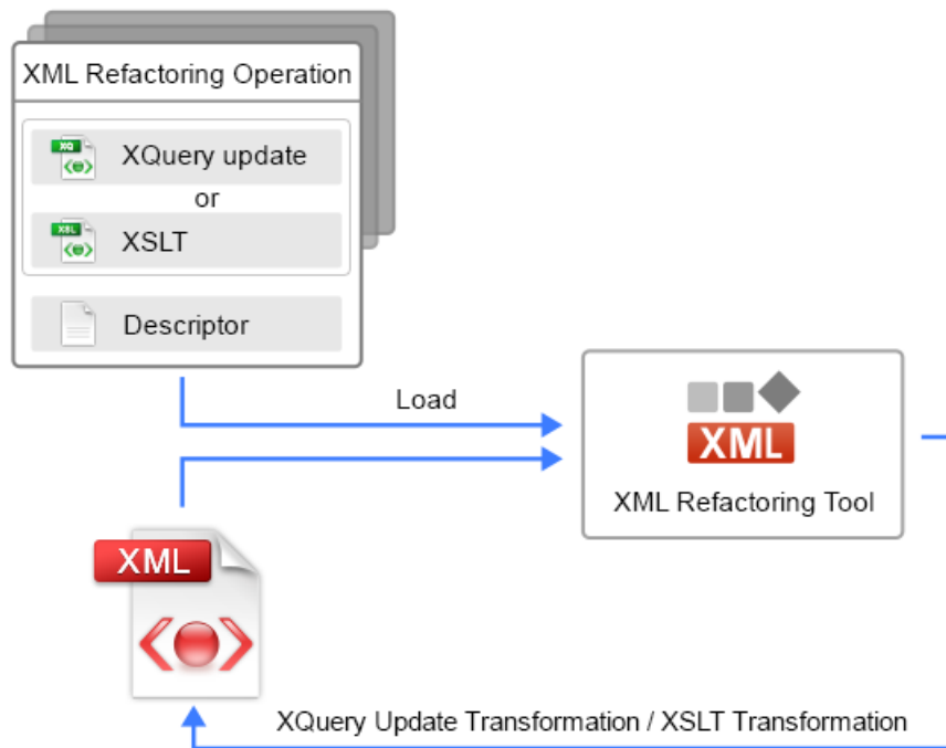
Figure 128: Diagram of an XML Refactoring Operation
