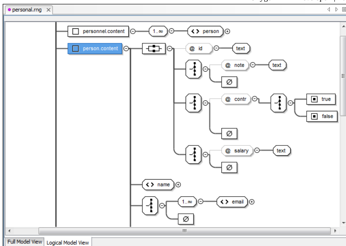
Figure 255: Logical Model View for a Relax NG Schema
