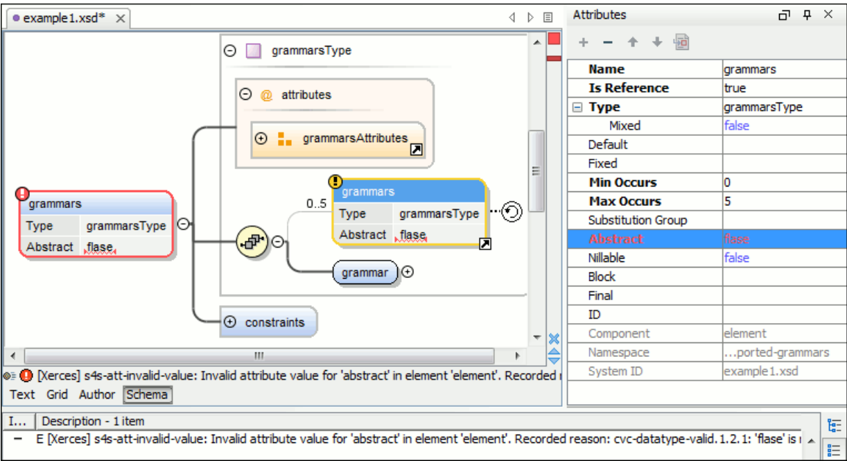
Figure 206: XML Schema Validation
