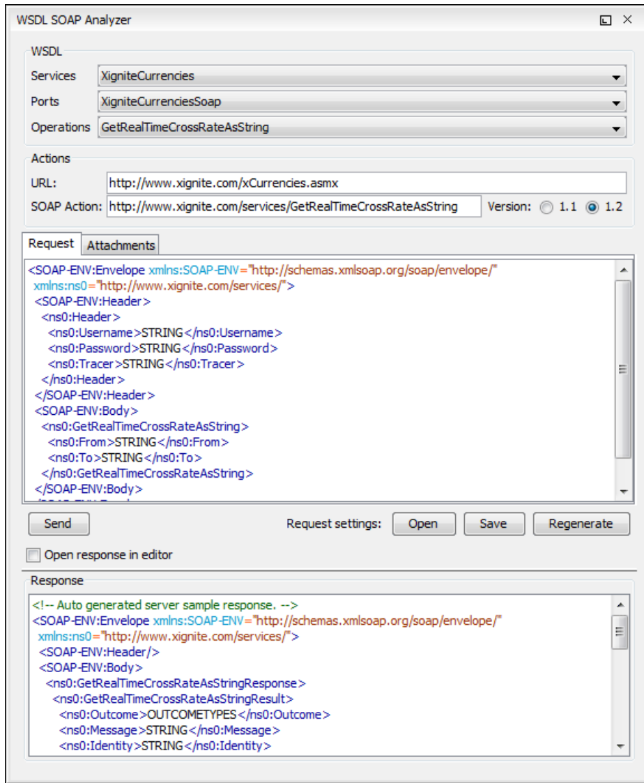
Figure 249: WSDL SOAP Analyzer Dialog Box
