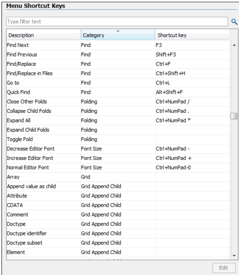
Figure 354: The Menu Shortcut Keys Preferences Panel
