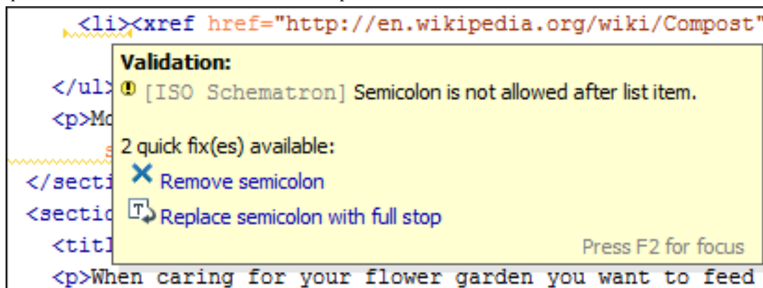
Figure 73: Quick Fix Presented in a Tooltip in Text Mode
