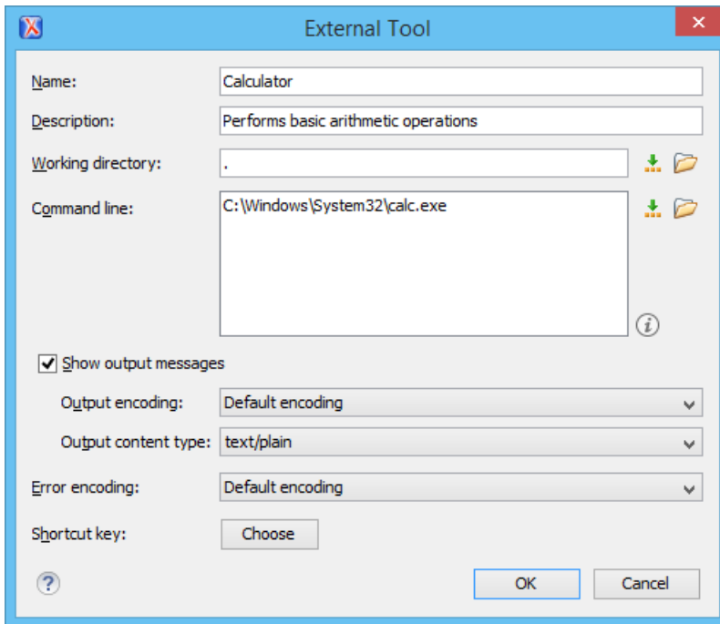
Figure 353: The External Tools Configuration Dialog Box
