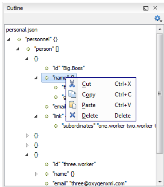
Figure 203: The JSON Outline View
