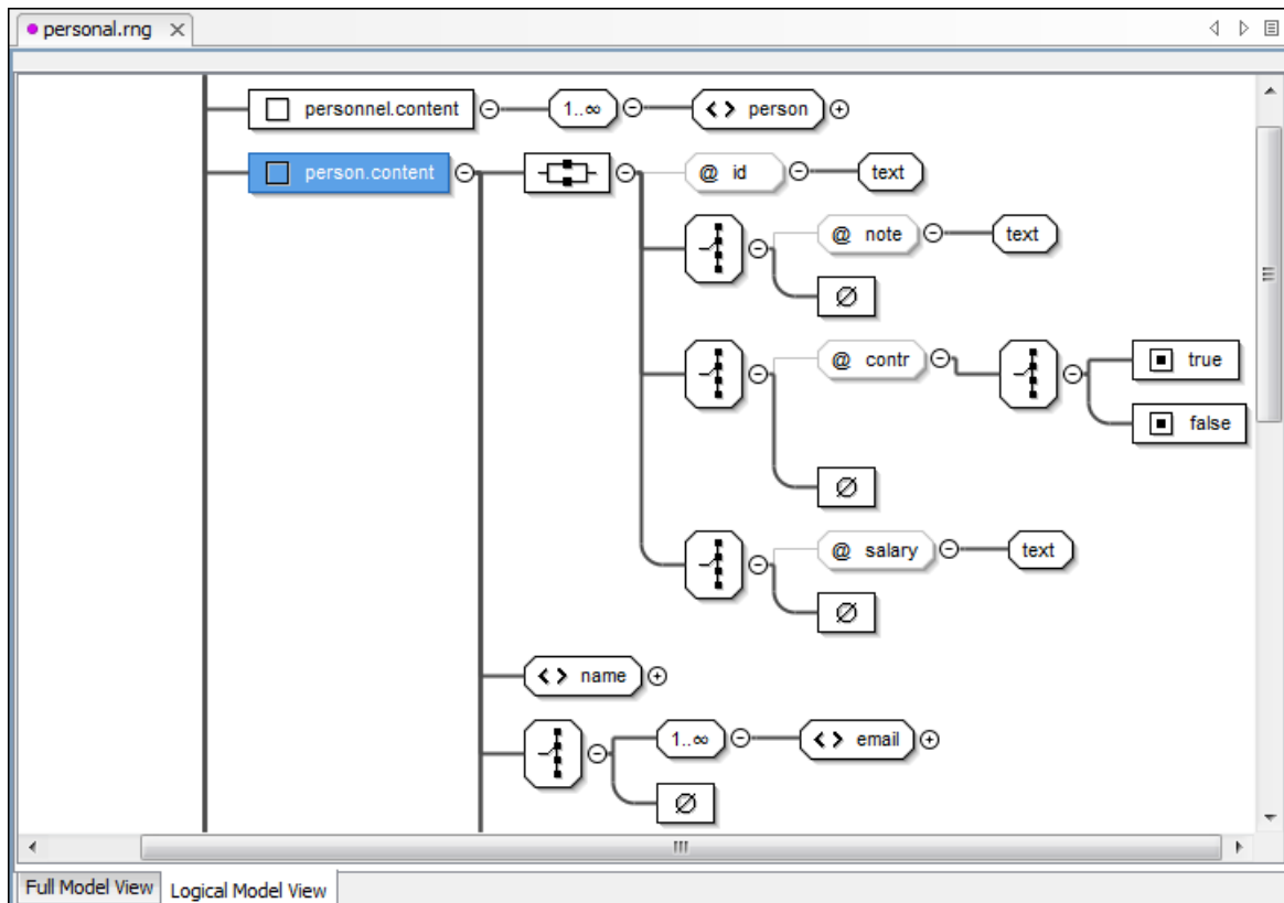
Figure 193: Logical Model View for a Relax NG Schema
