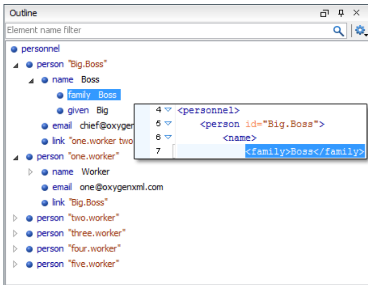
Figure 101: The Outline View
