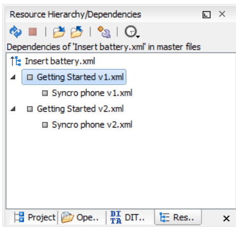
Figure 104: Resource Hierarchy/Dependencies View - Dependencies for Insert battery.xml
