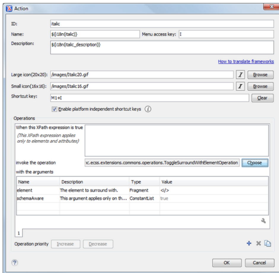
Figure 425: The Action Dialog
