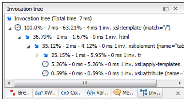
Figure 321: Invocation tree view
