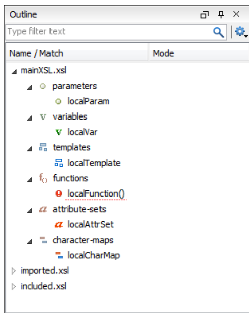
Figure 124: The XSLT Outline View
