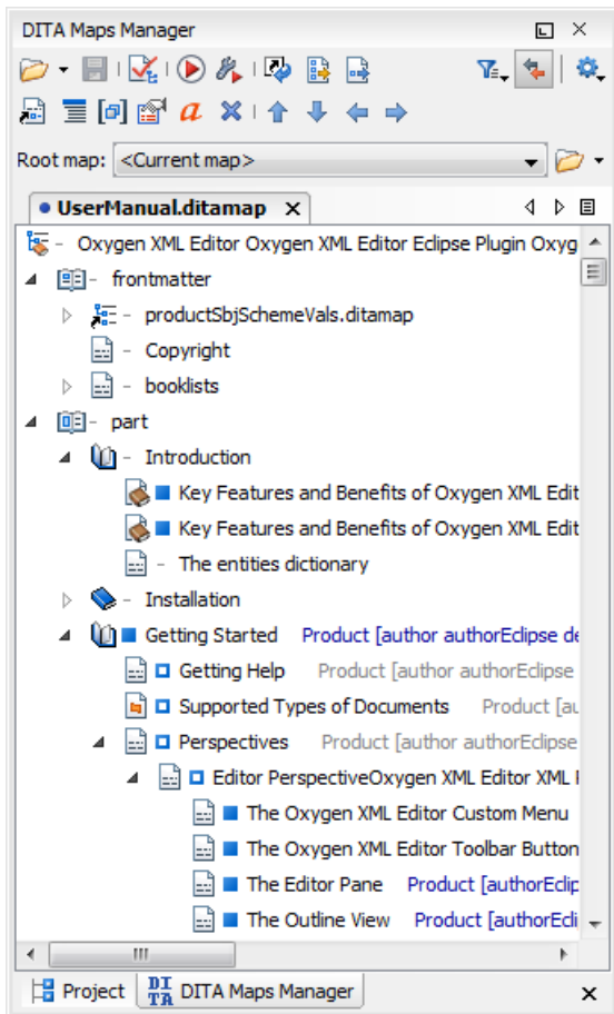
Figure 217: The DITA Maps Manager View
