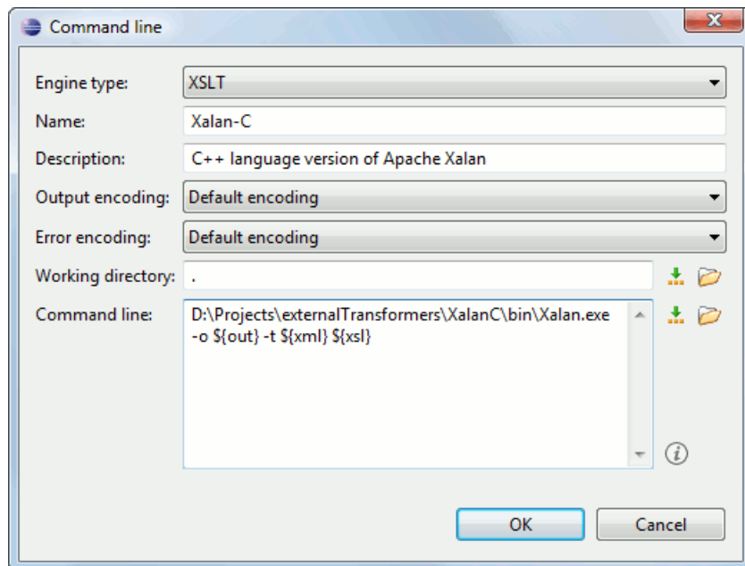
Figure 210: Parameters of a Custom Engine
