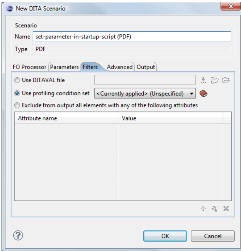
Figure 95: Edit Filters tab
