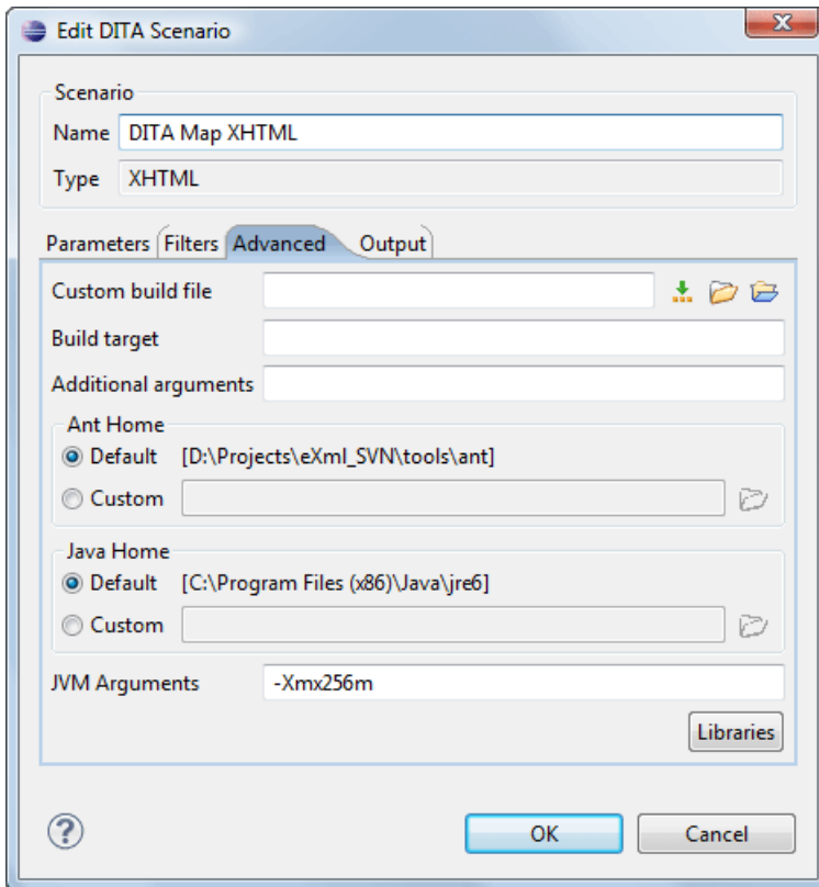
Figure 96: Advanced settings tab
