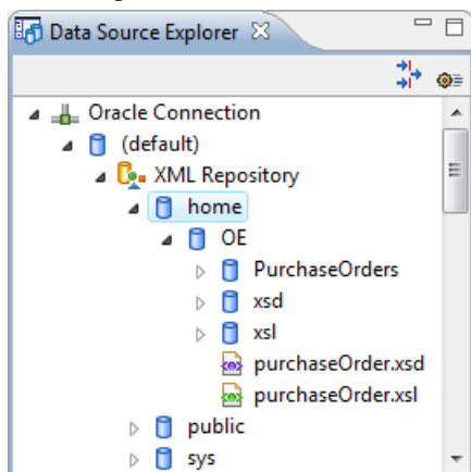
Figure 184: Browsing the Oracle XML DB Repository
