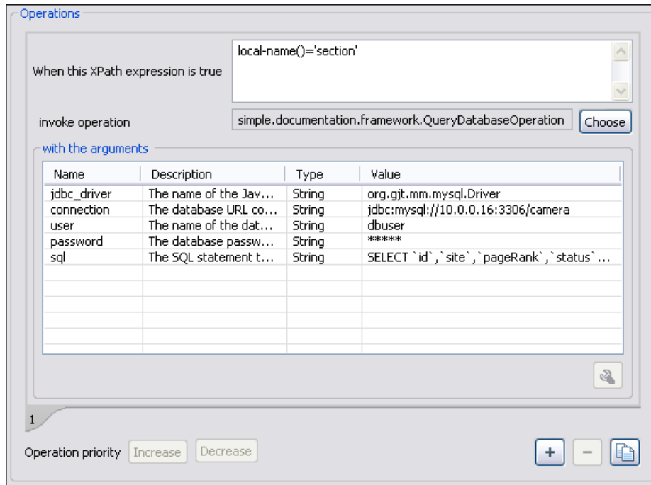
Figure 135: Java Operation Arguments Setup
