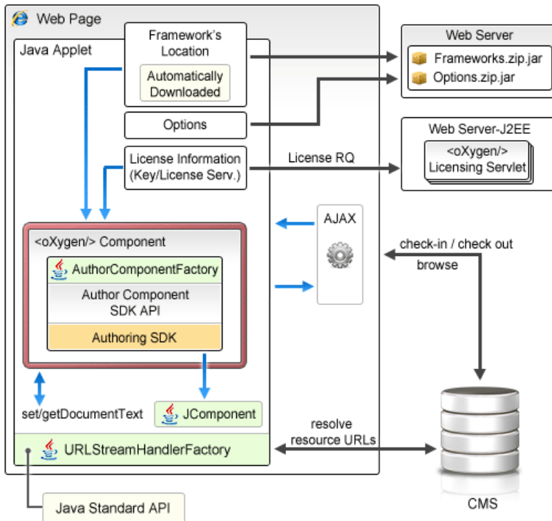
Figure 152: Oxygen XML Author plugin Author Component deployed as a Java applet
