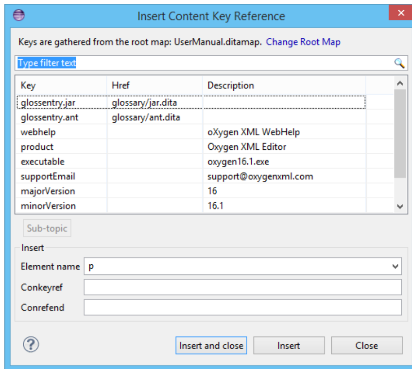
Figure 116: Insert Content Key Reference Dialog
