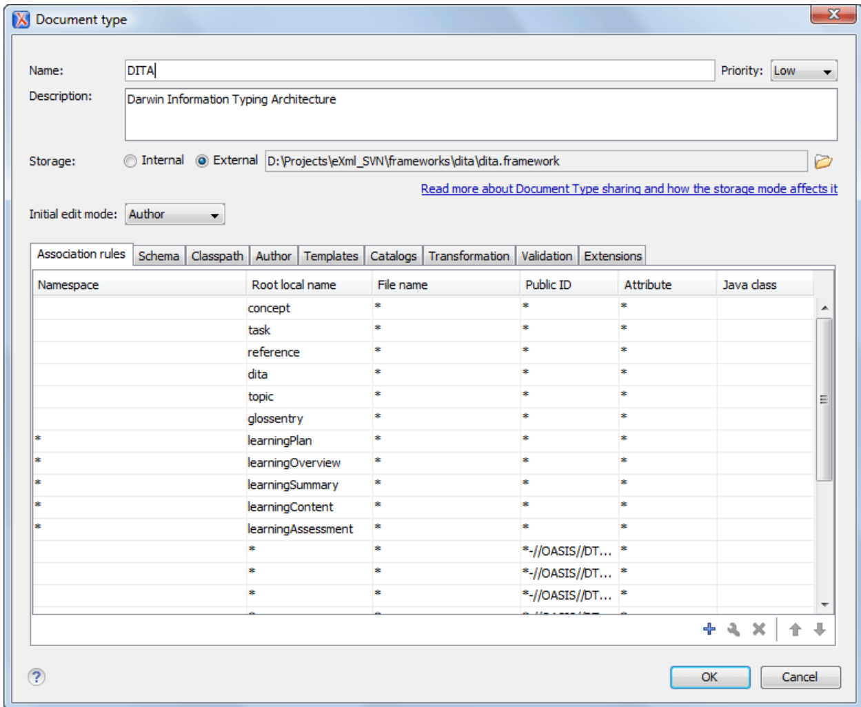
Figure 124: The Document Type
