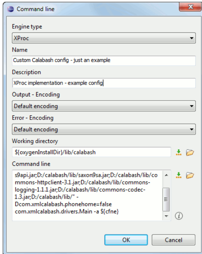
Figure 205: Creating an XProc external engine
