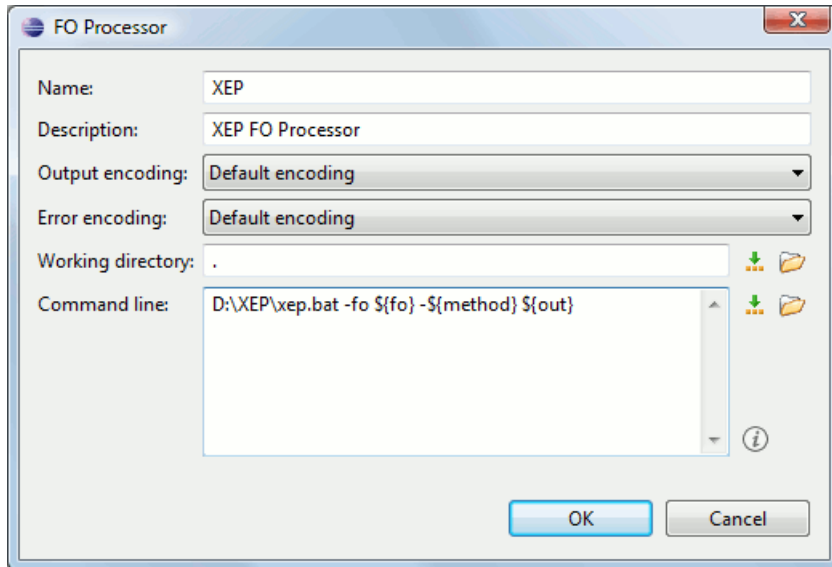
Figure 209: The External FO Processor Configuration Dialog
