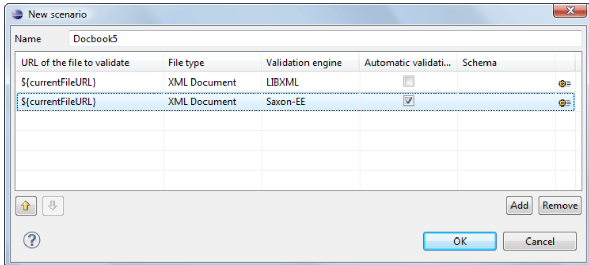
Figure 142: Add / Edit a Validation Unit
