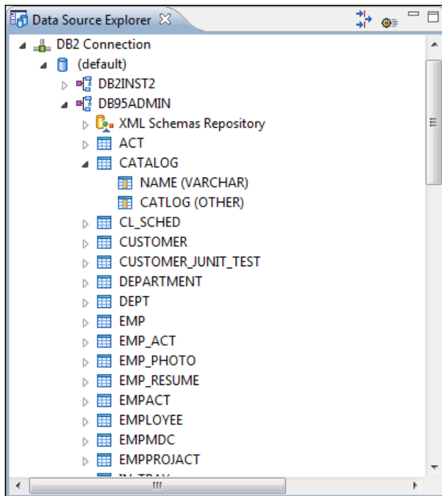
Figure 183: Data Source Explorer View
