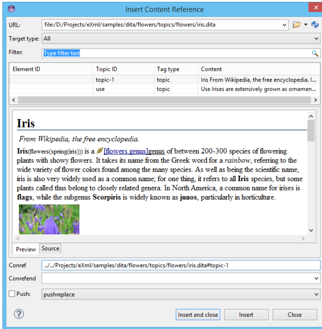
Figure 115: Insert Content Reference Dialog
