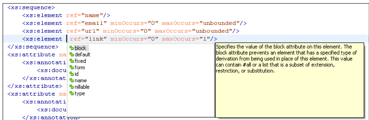
Figure 64: Content Completion Assistant
