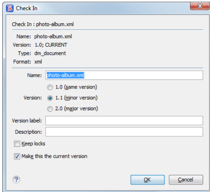
Figure 190: Check In Dialog
