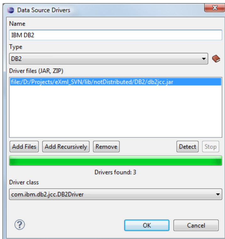
Figure 167: Data Source Drivers Configuration Dialog
