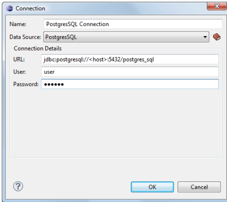
Figure 179: The Connection Configuration Dialog
