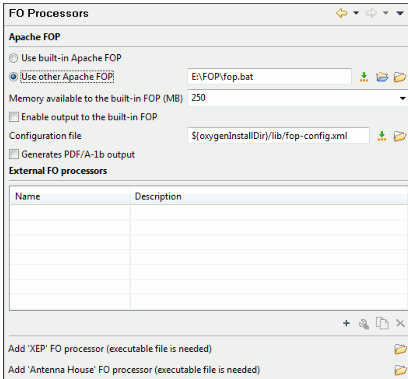
Figure 208: The FO Processors Preferences Panel
