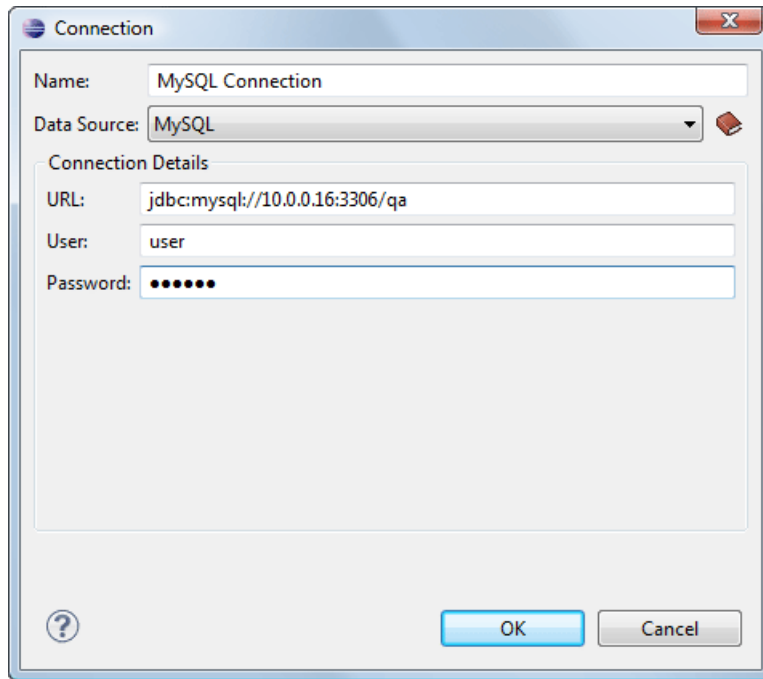
Figure 177: The Connection Configuration Dialog
