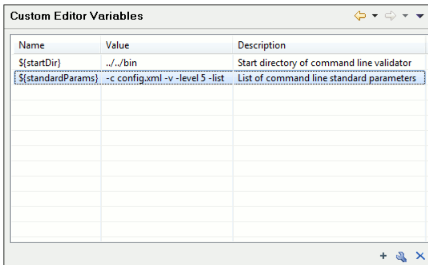
Figure 195: Custom Editor Variables
