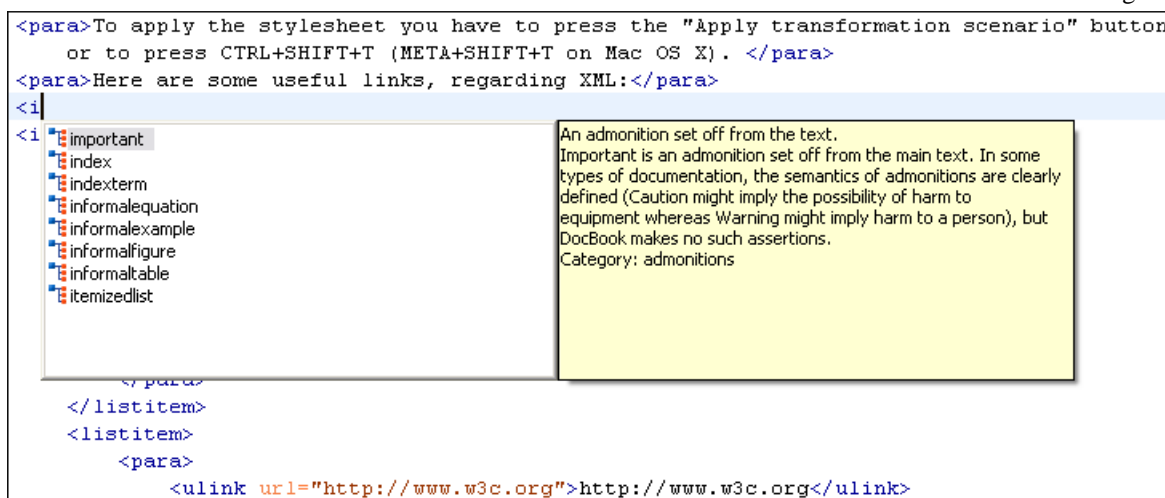
Figure 17: Content Completion Driven by DocBook DTD
