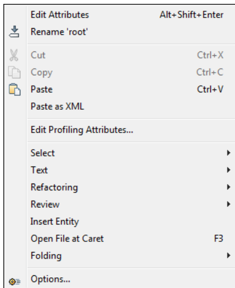
Figure 53: Contextual menu
