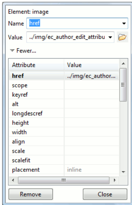
Figure 43: Edit attributes in place - full version
