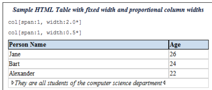
Figure 58: HTML table
