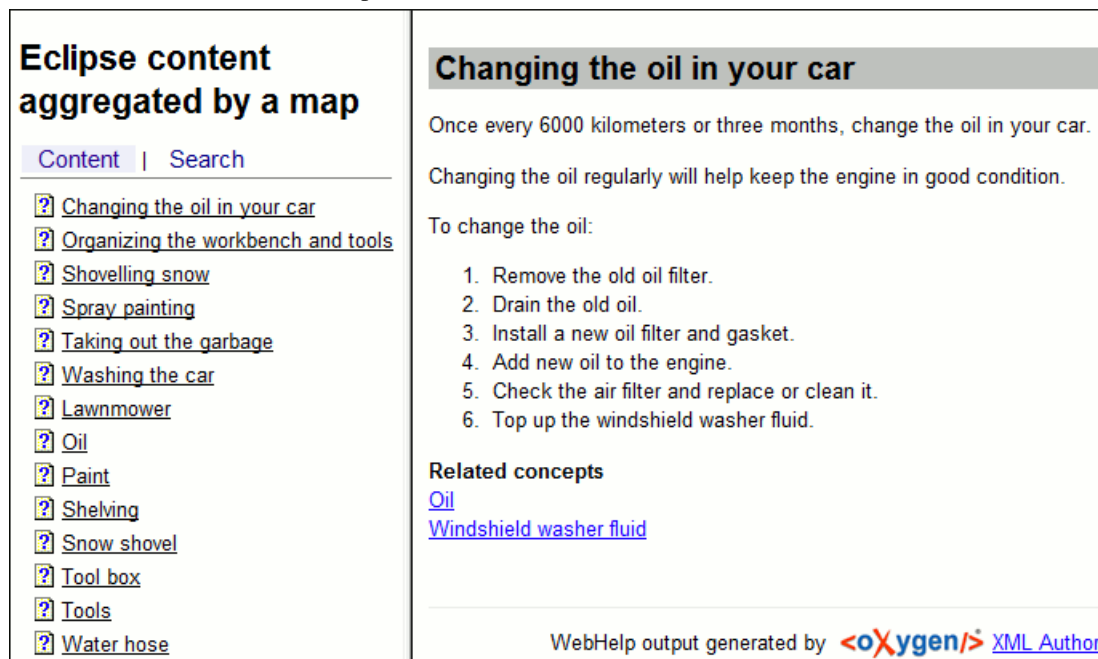
Figure 69: WebHelp Output
