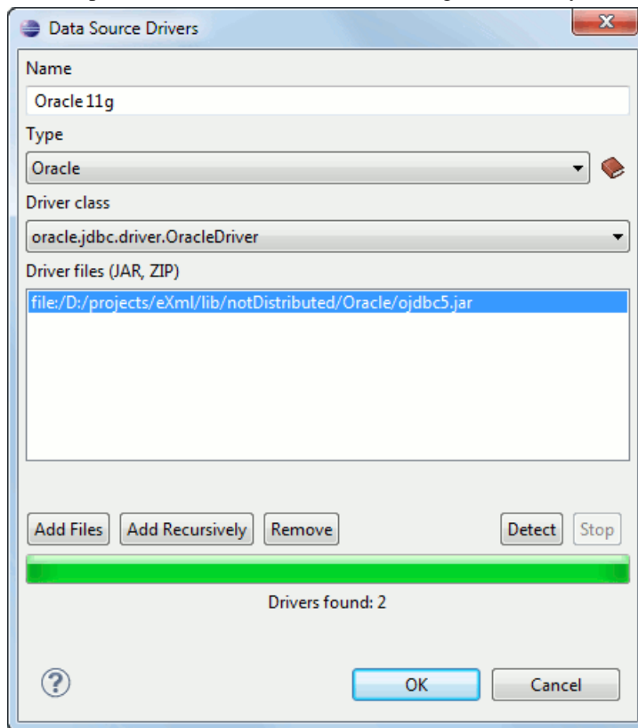
Figure 180: The Data Sources Drivers Dialog
