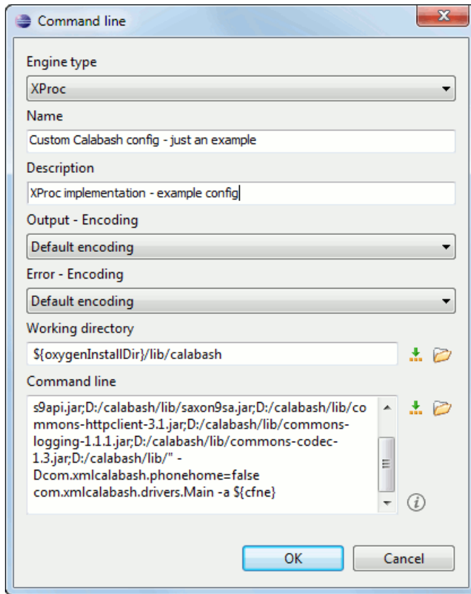
Figure 172: Creating an XProc external engine
