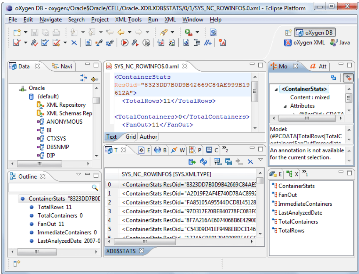
Figure 10: Database perspective
