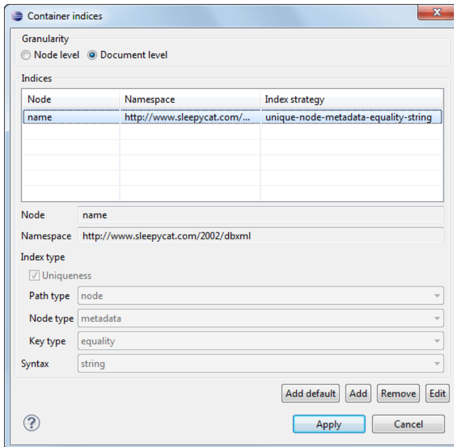
Figure 160: Container indices
