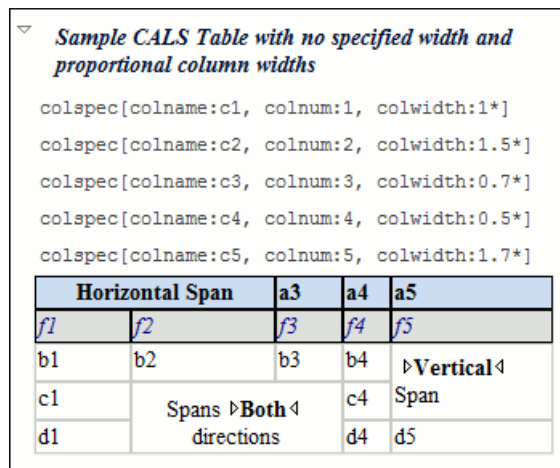
Figure 57: CALS table
