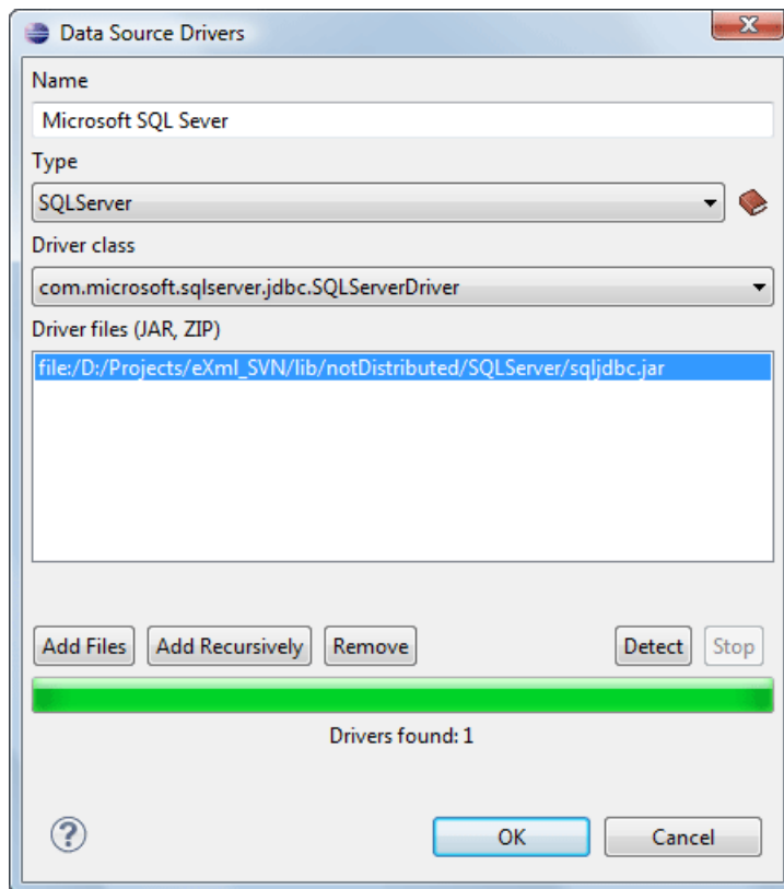
Figure 142: Data Source Drivers Configuration Dialog
