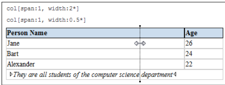
Figure 56: Resizing a column in Oxygen XML Author plugin Author editor
